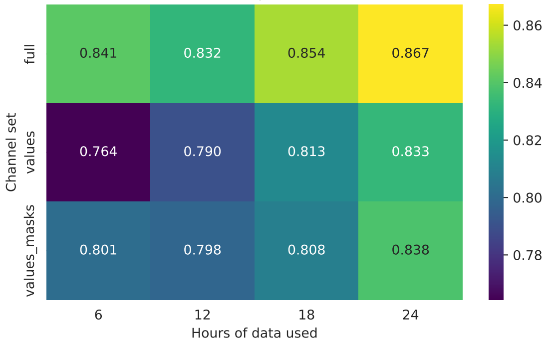
Best Test AUPRC per ablation cell
