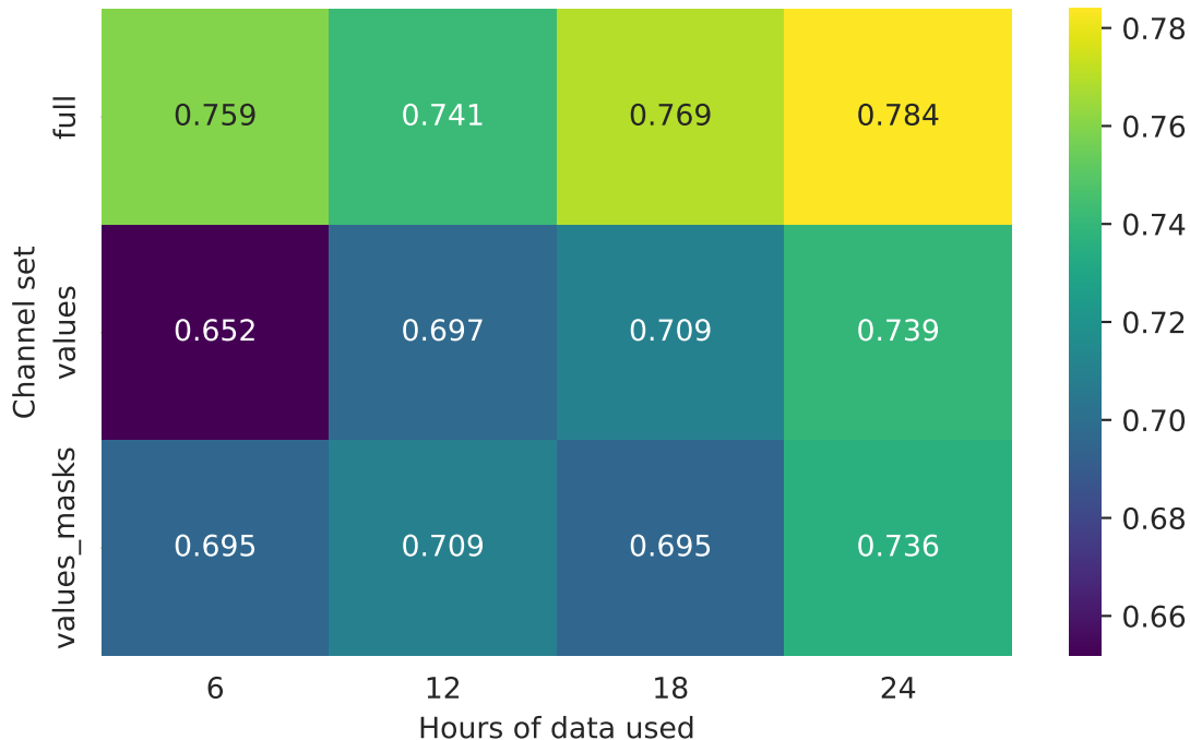
Best Test AUROC per ablation cell
