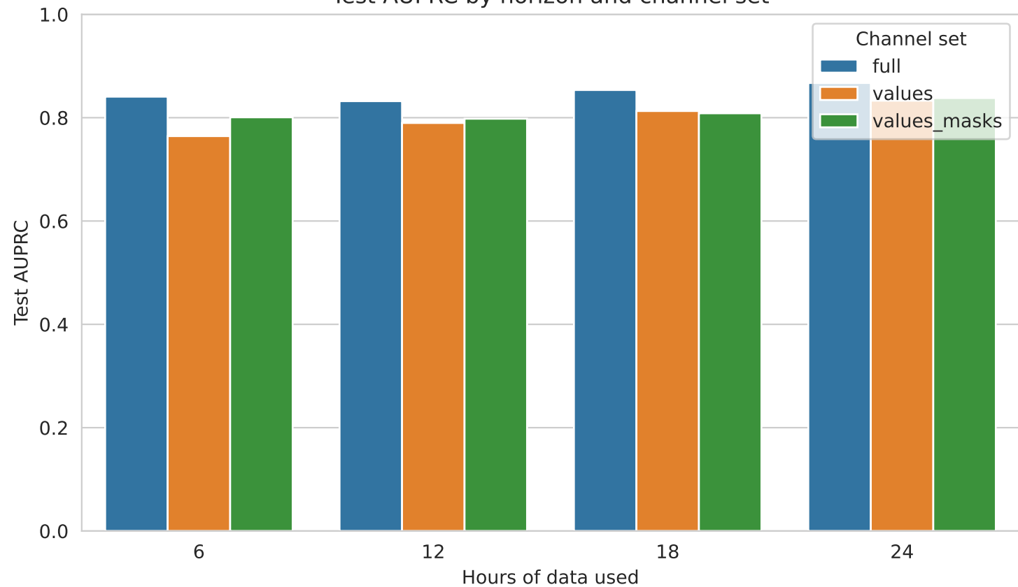
Test AUPRC by horizon and channel set
