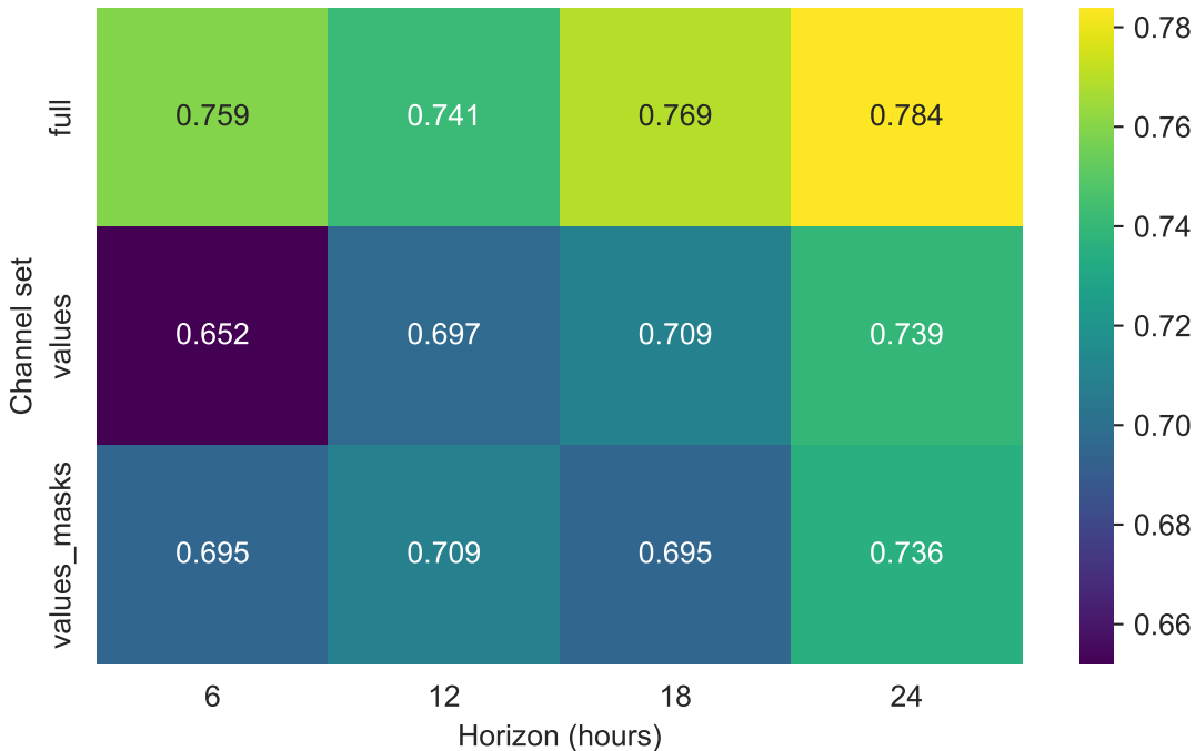
cnn_bdlstm: best Test AUROC per horizon/channel set
