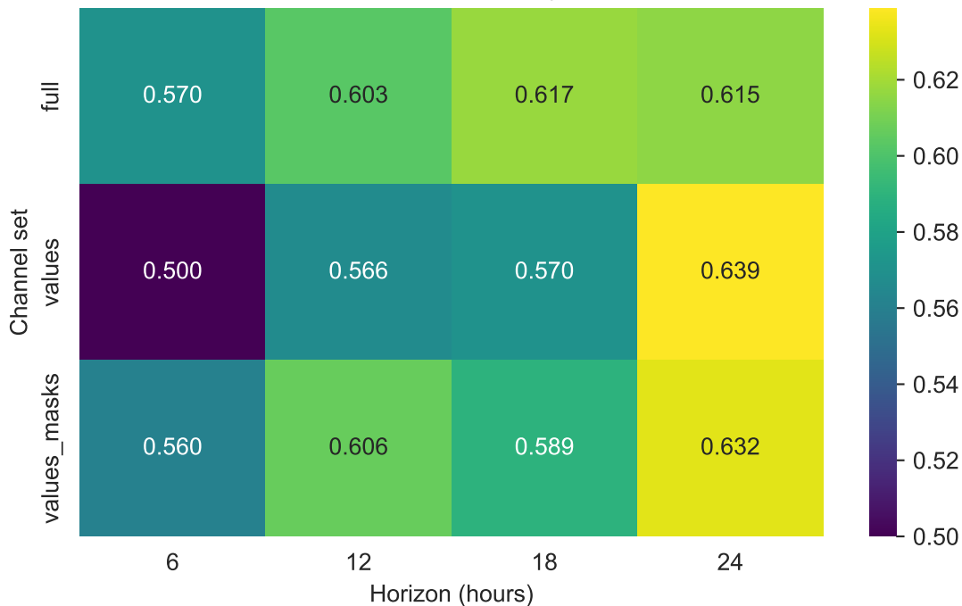
cnn_bdlstm: best Test Balanced Accuracy per horizon/channel set
