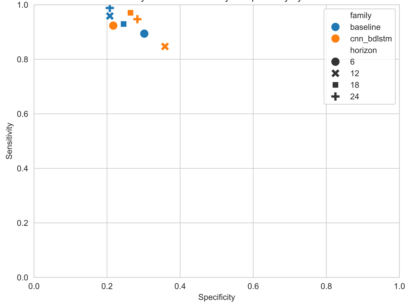
Best Family Models: Sensitivity vs Specificity by Horizon
