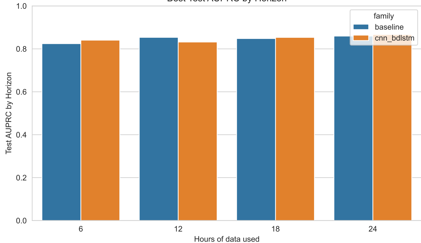
Best Test AUPRC by Horizon
