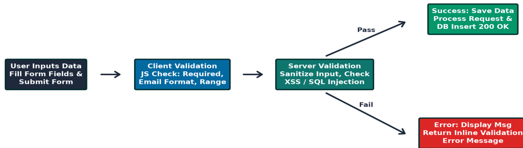
Diagram: Web Form Input Validation & Security Lifecycle.
