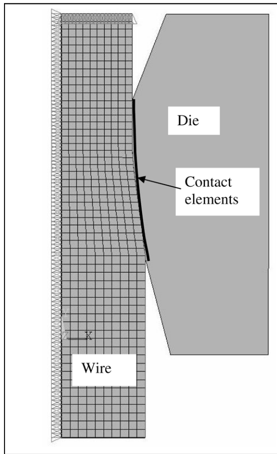
Fig. 3. Finite element model.
