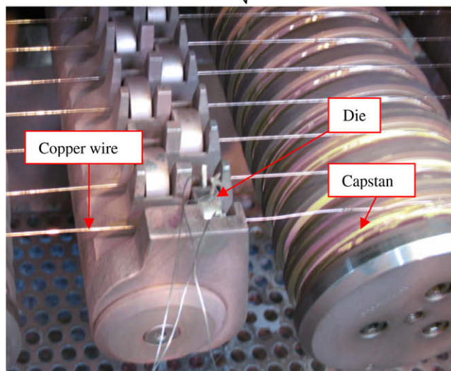
Fig. 2. Multipass drawing machine and principal equipment.
