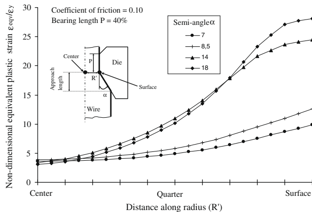
Fig. 7. Ratio of equivalent plastic strain to initial yield strain versus distance along radius at the exit of the die.
