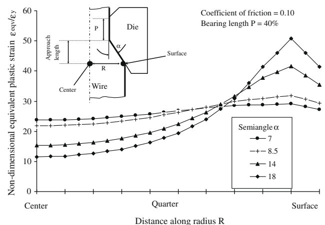
Fig. 6. Ratio of equivalent plastic strain to initial yield strain versus distance along radius at the entrance of the die.
