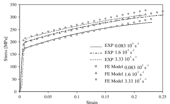
Fig. 1. Stress-strain curves of copper wire in various speeds.
