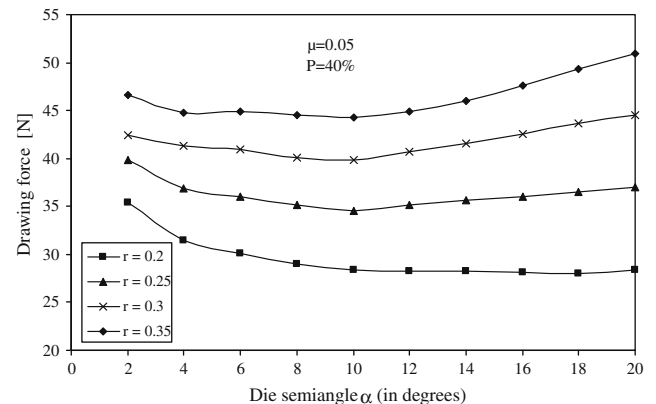
Fig. 5. Variation of drawing force with die-angle at different reductions.
