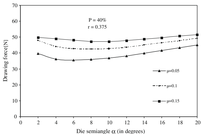
Fig. 4. Drawing force obtained from FEM analysis.
