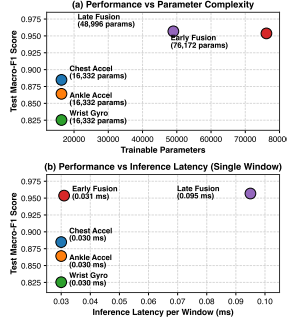
Figure 8: Embedded deployment trade-offs: (a) Macro-F1 vs Trainable Parameters; (b) Macro-F1 vs Single-Window Inference Latency (ms).
