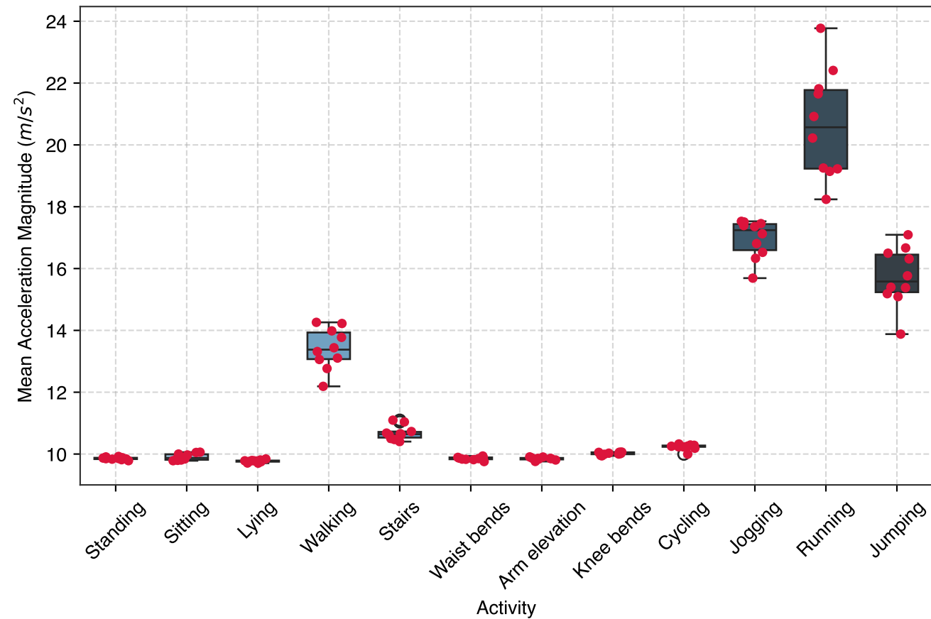
(a) Ankle Acceleration Magnitude across Activities (10 Subjects)
