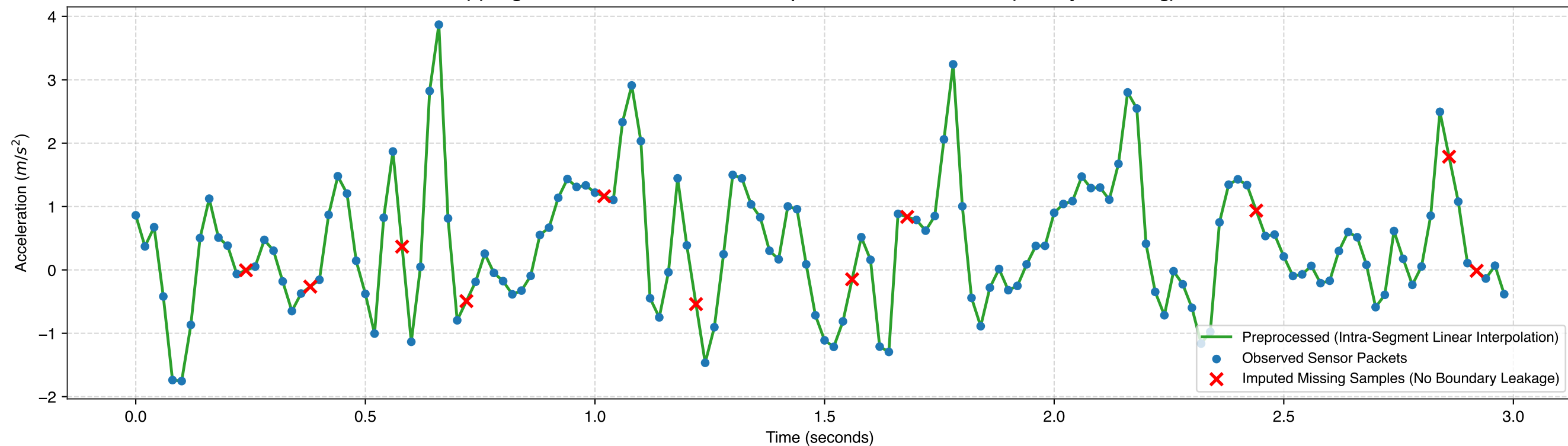
(c) Segment-Bounded Time-Series Interpolation on Chest Accel-Y (Activity 4: Walking)
