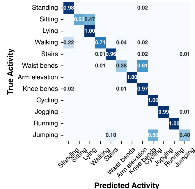
Wrist Gyro (Acc: 85.6%, F1: 0.825)
