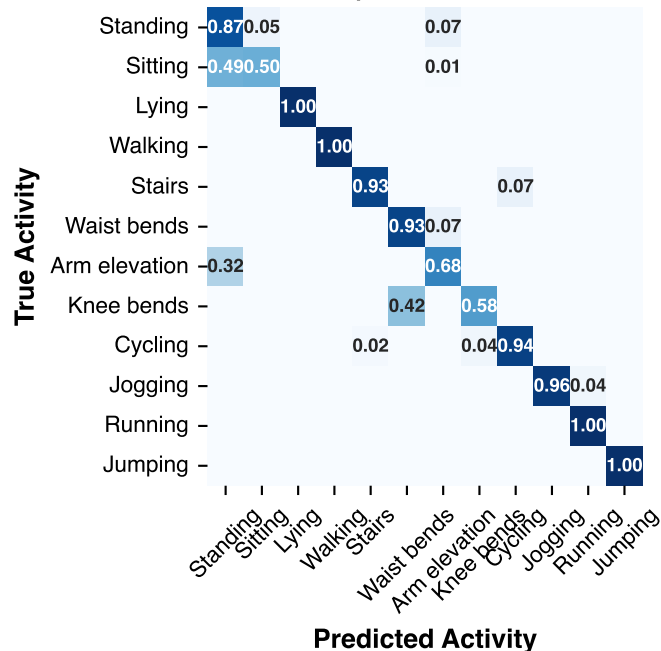
Ankle Accel (Acc: 85.9%, F1: 0.864)
