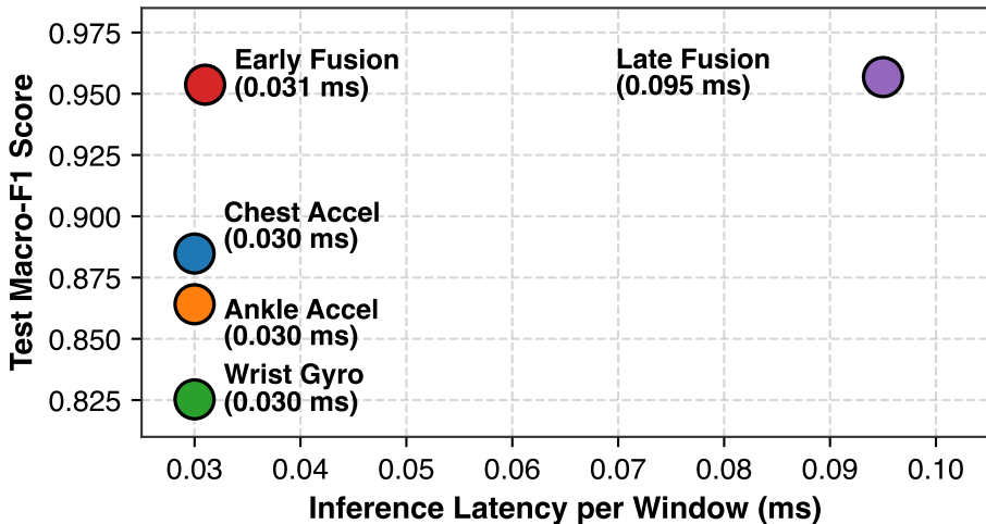
(b) Performance vs Inference Latency (Single Window)
