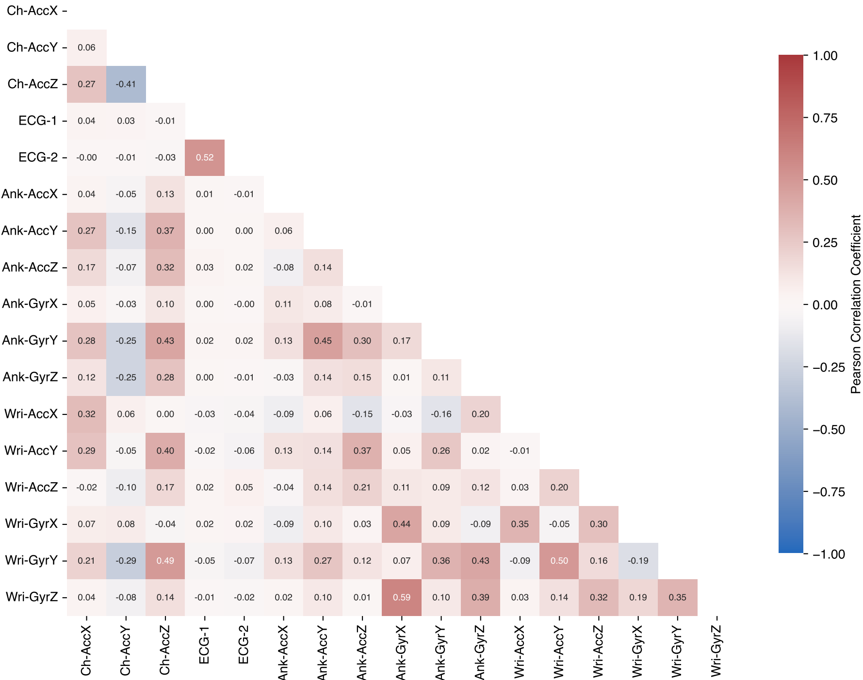
Cross-Sensor & Cross-Modality Correlation Matrix (MHEALTH)
