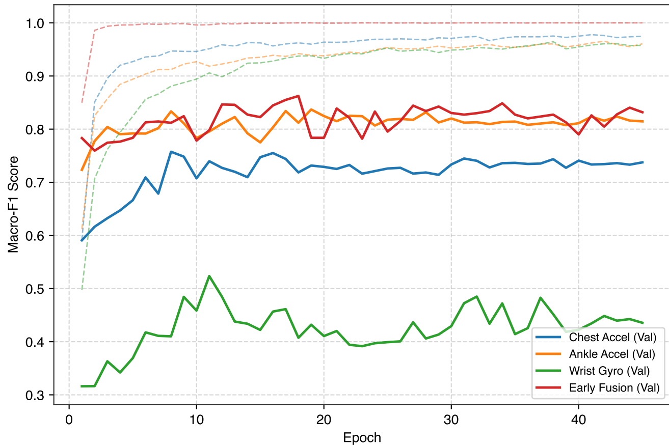
(b) Training (dashed) & Validation (solid) Macro-F1
