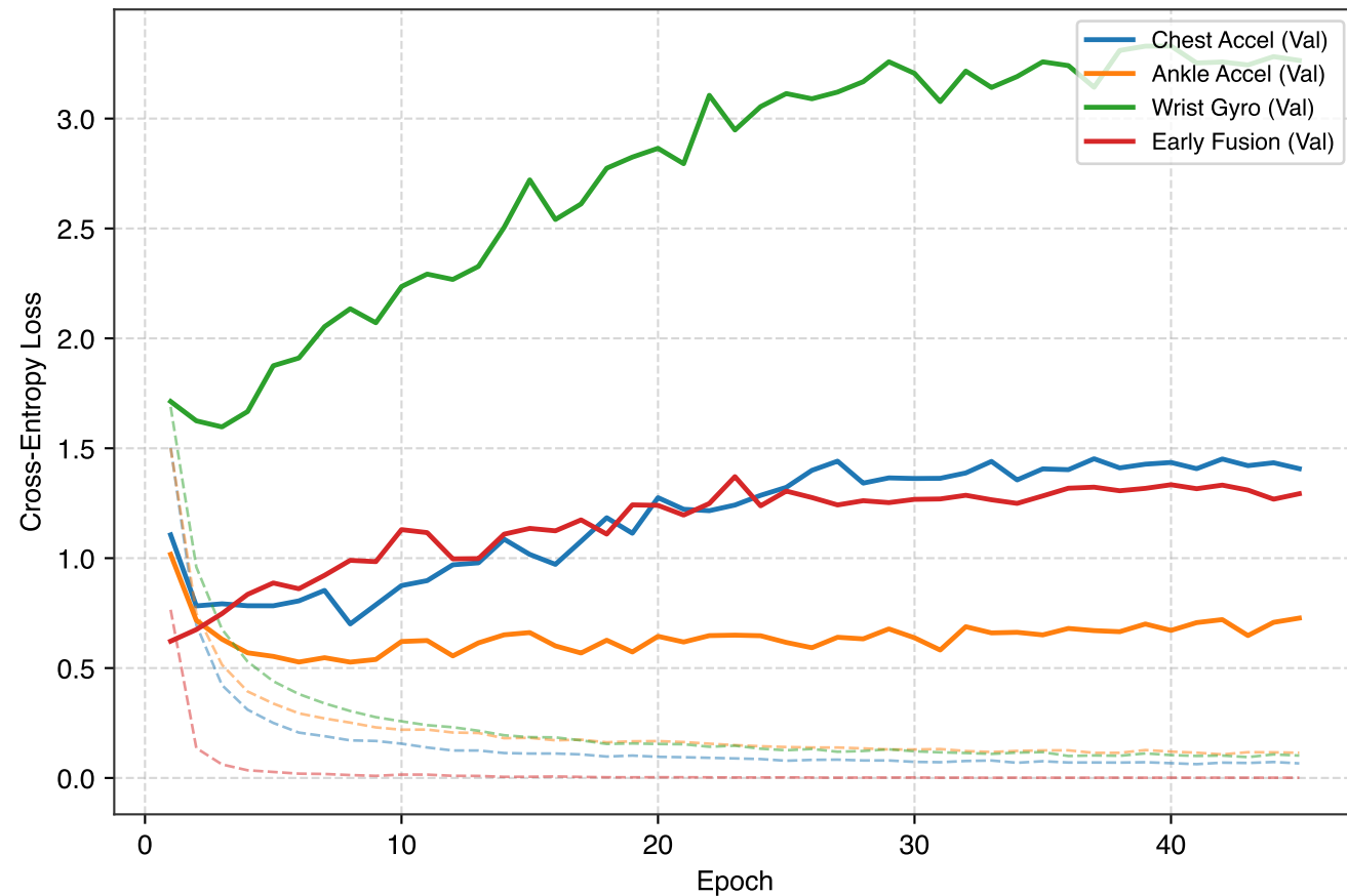
(a) Training (dashed) & Validation (solid) Loss
