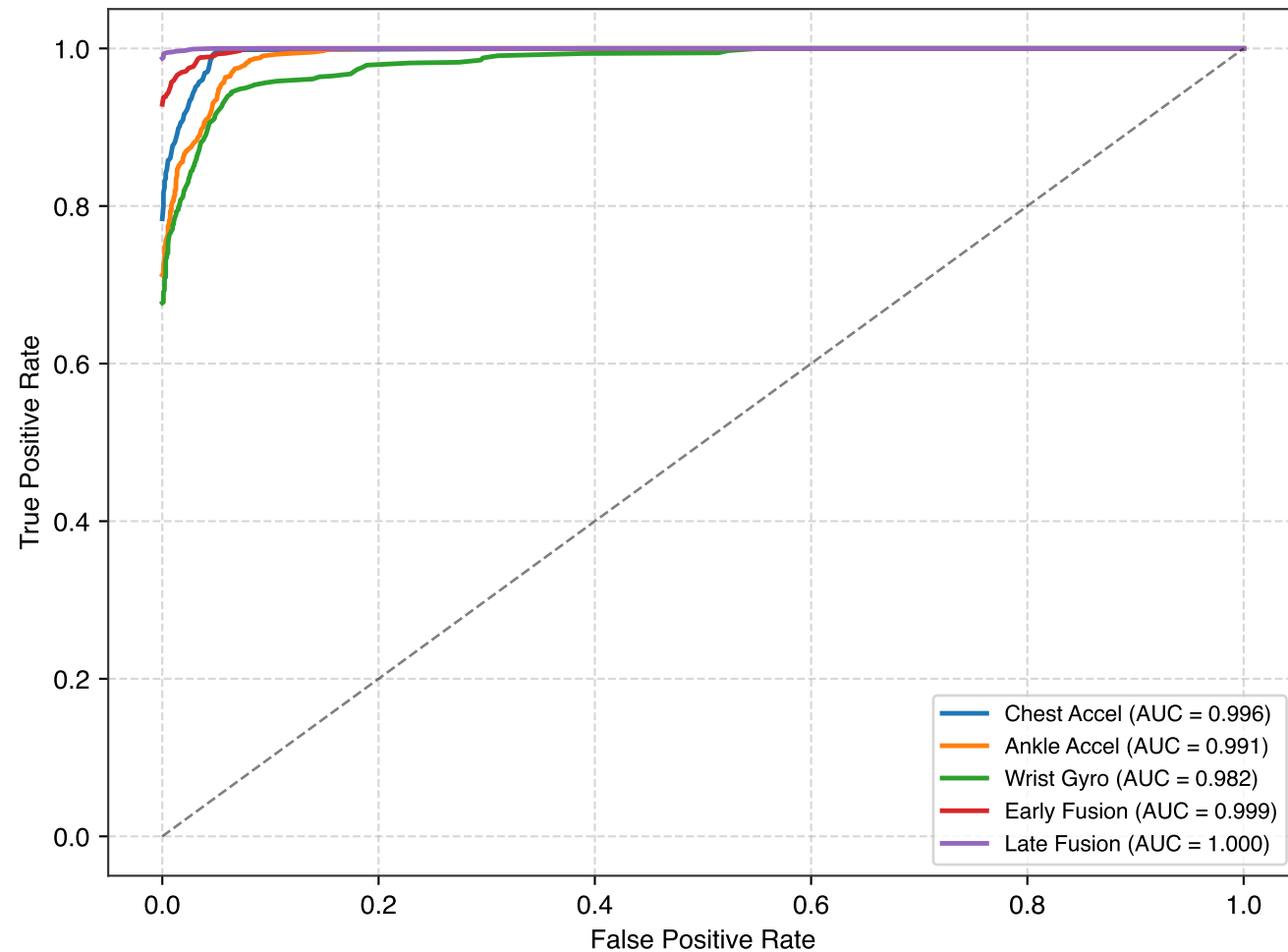
(a) Macro-Average Receiver Operating Characteristic (ROC)
