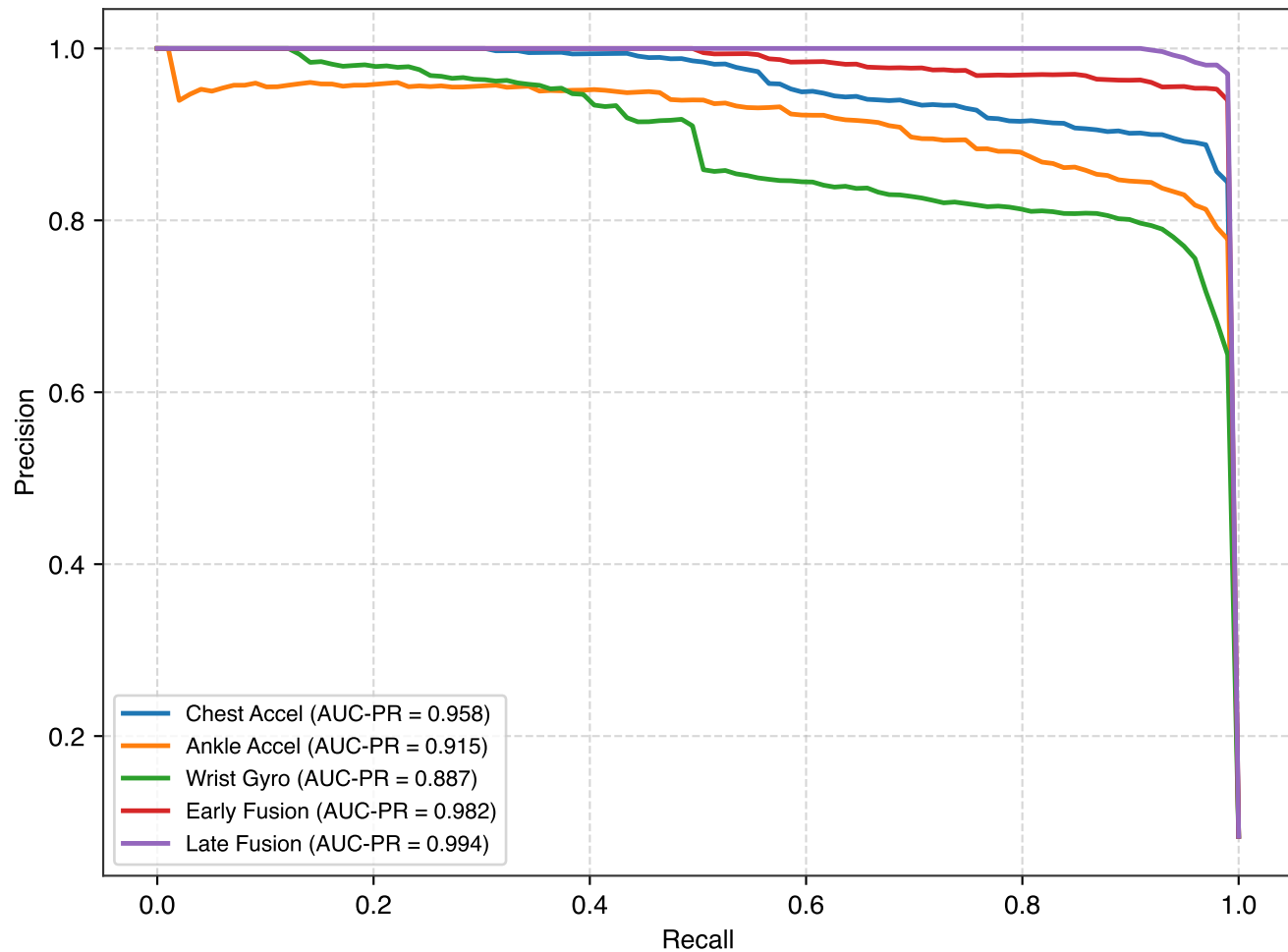
(b) Macro-Average Precision-Recall (PR) Curves
