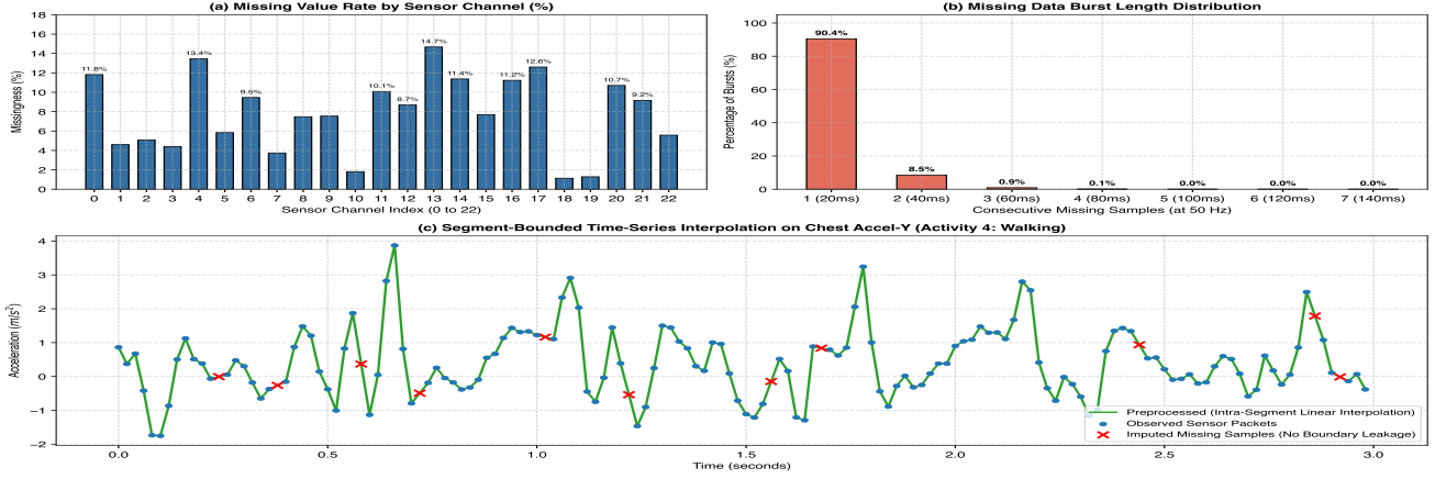
Figure 4: Missing data audit and preprocessing pipeline: (a) Percentage missingness per sensor channel (Channels 0–22); (b) Burst length frequency distribution, confirming 90.4% single-sample drops (20 ms); (c) Intra-segment linear interpolation on Chest Accel-Y during Walking ( L_4 ), demonstrating accurate trajectory reconstruction without cross-activity boundary leakage.
