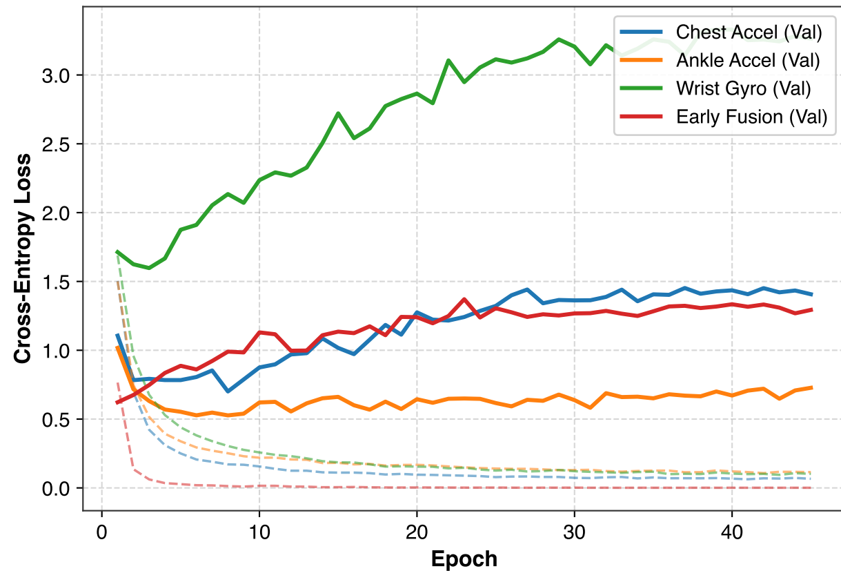
(a) Training (dashed) & Validation (solid) Loss
