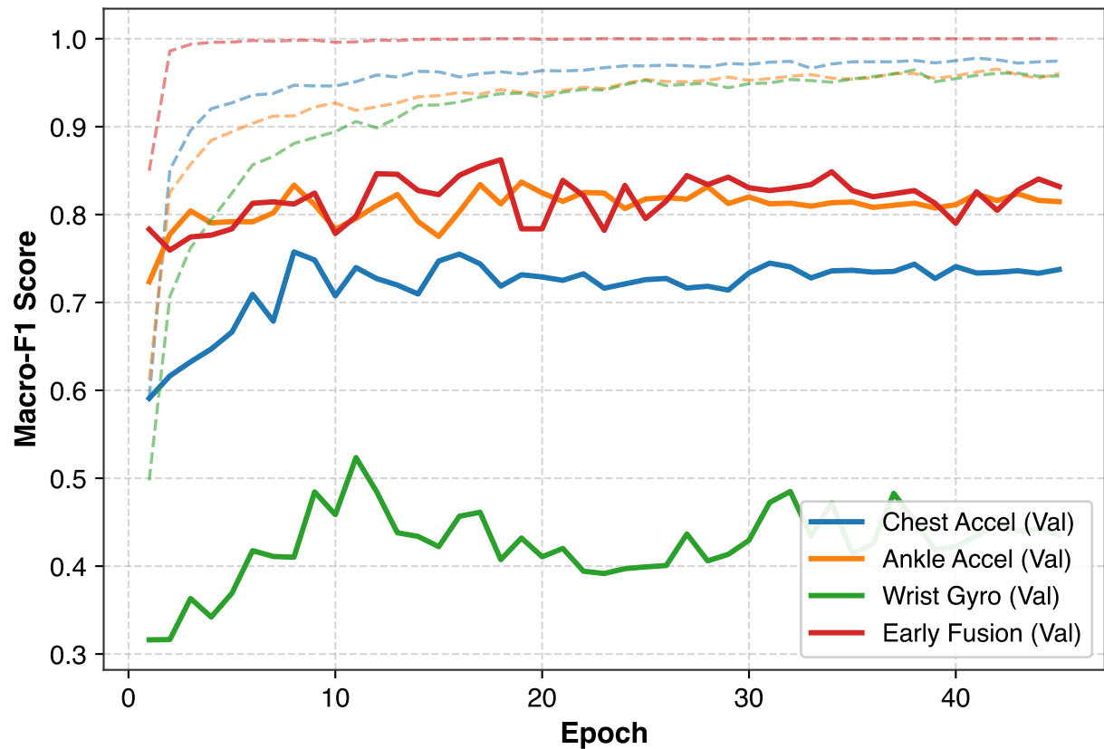
(b) Training (dashed) & Validation (solid) Macro-F1
