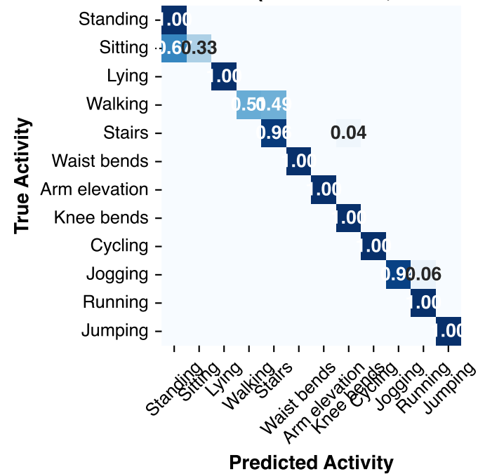
Early Fusion (Acc: 95.3%, F1: 0.954)
