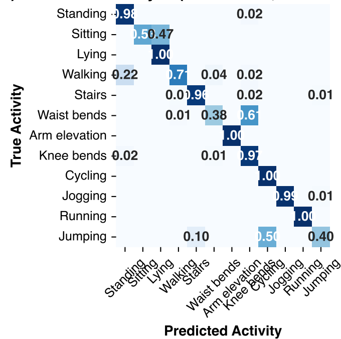
Wrist Gyro (Acc: 85.6%, F1: 0.825)
