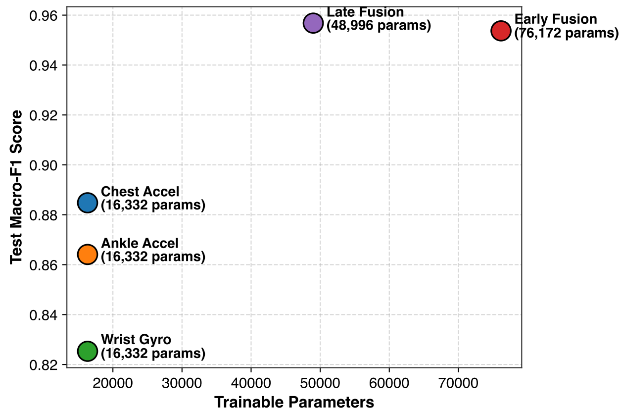
(a) Performance vs Parameter Complexity
