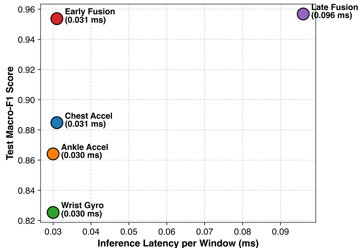
(b) Performance vs Inference Latency (Single Window)
