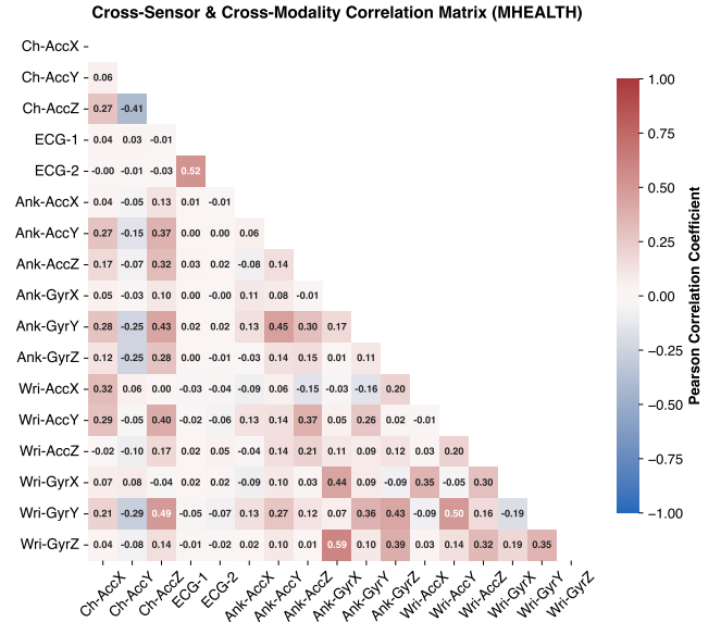
Figure 3: Cross-sensor Pearson correlation matrix across 17 kinematic and physiological channels ( N = 50,000 ).
