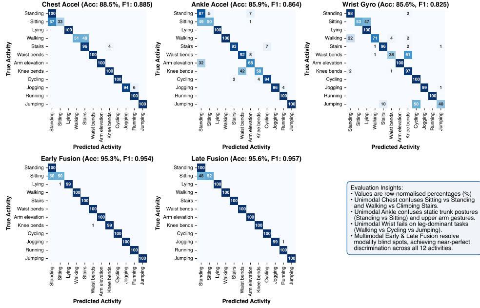
Figure 6: Normalized test-set confusion matrices across all five models ( N_{\text{test}} = 1,035 windows across unseen Subjects 9 and 10; values are row-normalised %), detailing how multimodal fusion resolves unimodal misclassifications across the 12 activity classes.
