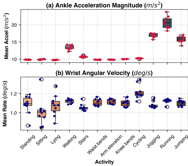
Figure 2: Kinetic energy distributions across 10 participants: (a) Mean Ankle Acceleration Magnitude ( m/s^2 ); (b) Mean Wrist Angular Velocity ( deg/s ). Points denote participant averages, illustrating inter-subject variation.
