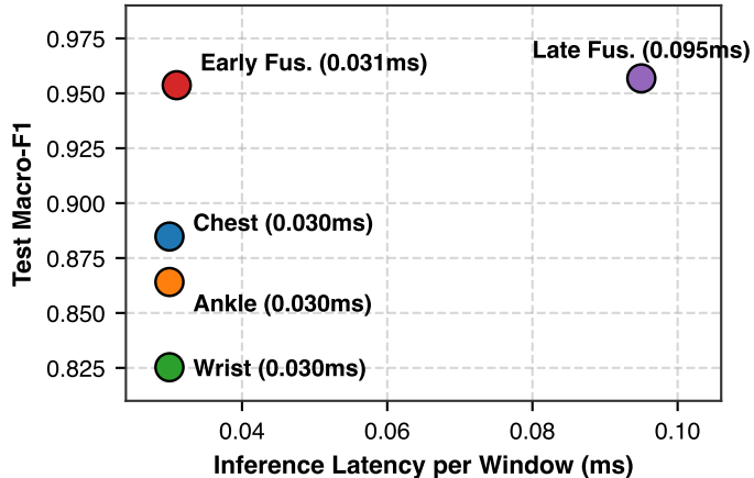
(b) Macro-F1 vs Latency
