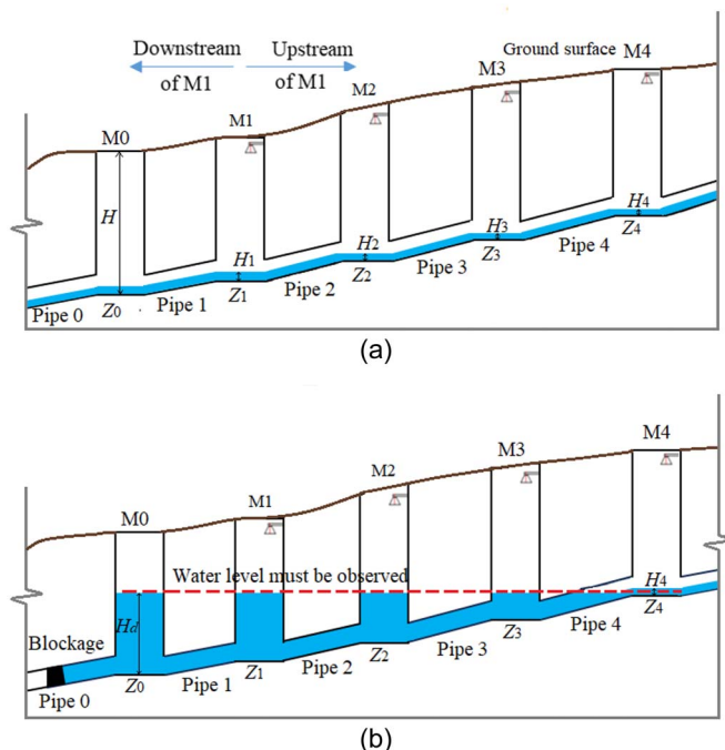
Fig. 3. Example of the blockage detection condition for sensor locations. Water level in (a) normal conditions; and (b) blockage conditions. In this example, sensors at M1, M2, and M3 can detect water level rise at an inspection hole M0 caused by a blockage occurring at Pipe 0, while the sensor at M4 cannot detect the blockage. M3 is the optimal location to install a sensor as it is the most distant sensor that can observe this blockage. Sensors at M1 and M2 are redundant in this context.
