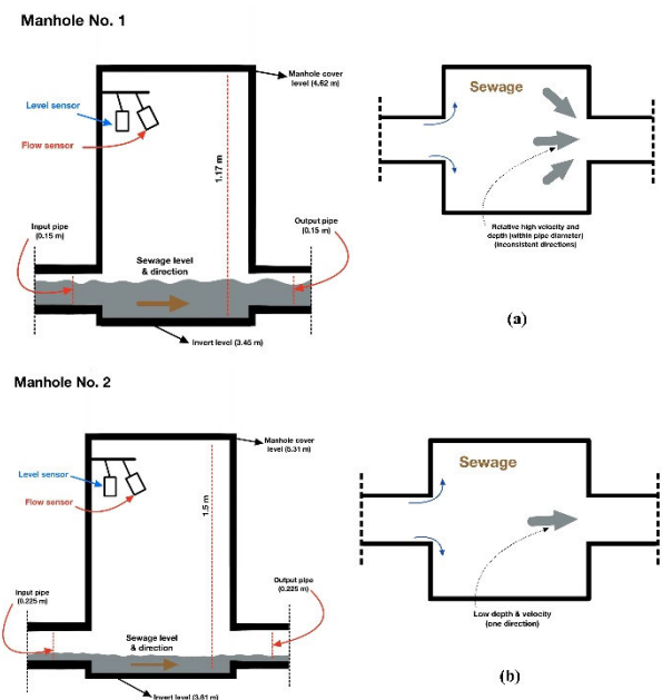
FIGURE 14. The effect of output pipe size in Two cases of flow sensor measurement (a) results in inaccurate values and (b) results in accurate values.
