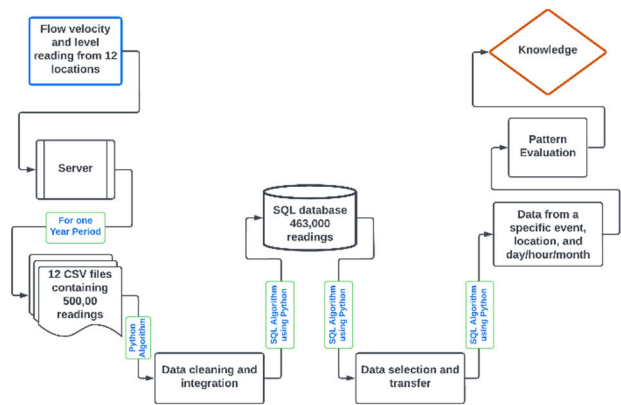
FIGURE 4. A flow chart depicts the data mining process used in this research.
