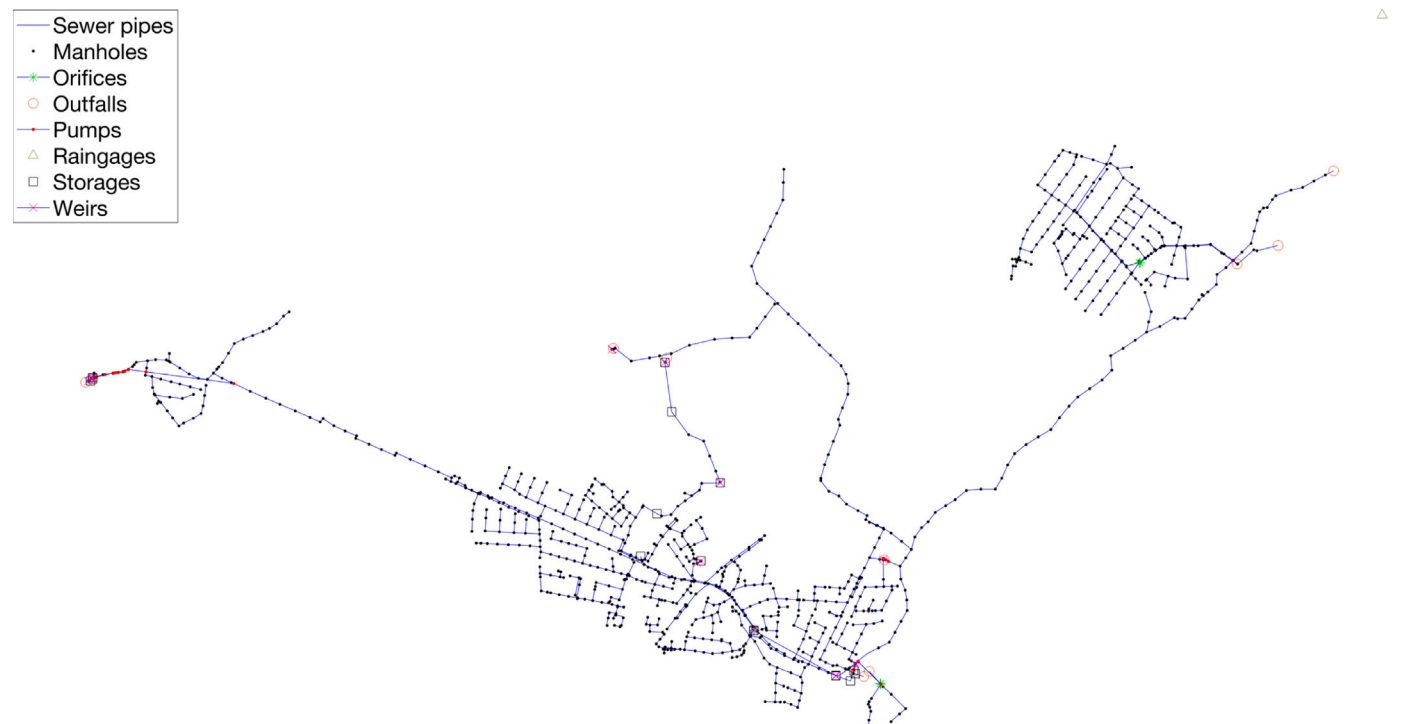
Fig. 4. Graph depicting Bellinge from the SWMM shape files.
