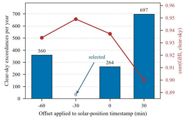
FIGURE 2. Clear-sky exceedances (bars, left axis) and correlation with the clear-sky reference (line, right axis) against the offset applied to the solar-position timestamp.
