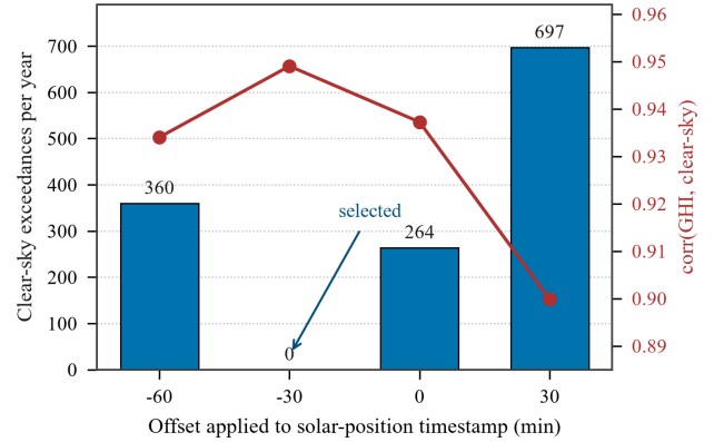
FIGURE 2. Clear-sky exceedances (bars, left axis) and correlation with the clear-sky reference (line, right axis) against the offset applied to the solar-position timestamp.
