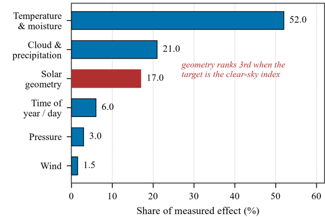
FIGURE 5. Grouped permutation importance for the clear-sky index target. Solar geometry (highlighted) ranks third.
