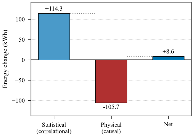
FIGURE 6. The learned correlational pathway and the causal physical pathway are of comparable magnitude and opposite sign; the net response conceals both.
