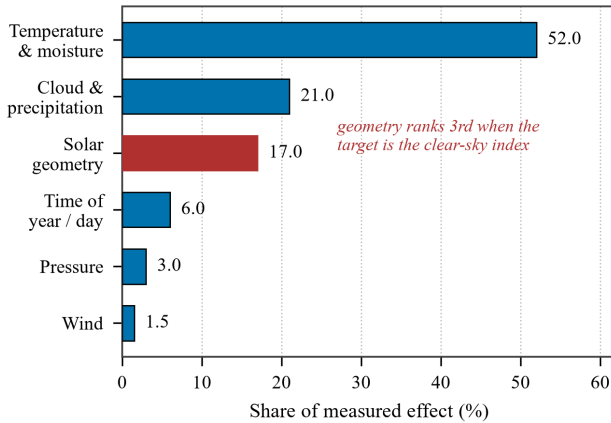
FIGURE 5. Grouped permutation importance for the clear-sky index target. Solar geometry (highlighted) ranks third.
