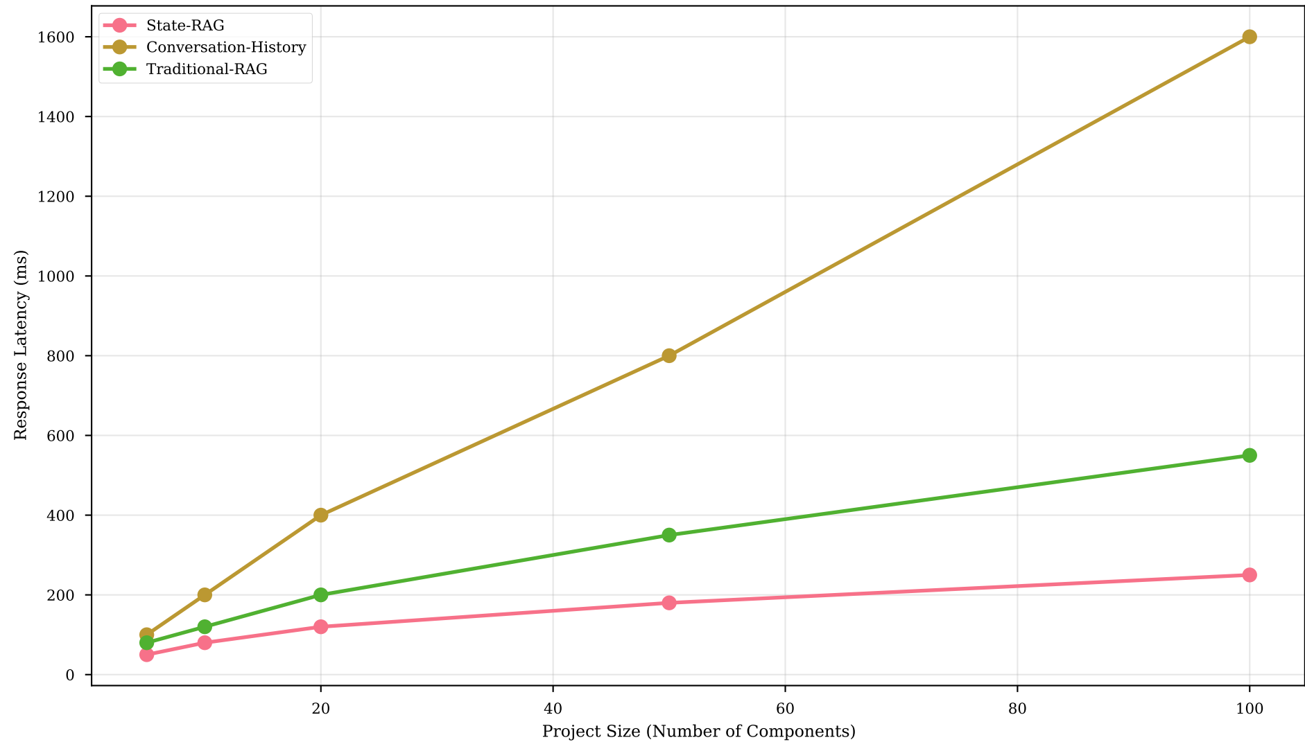
Scalability: Latency vs Project Size
