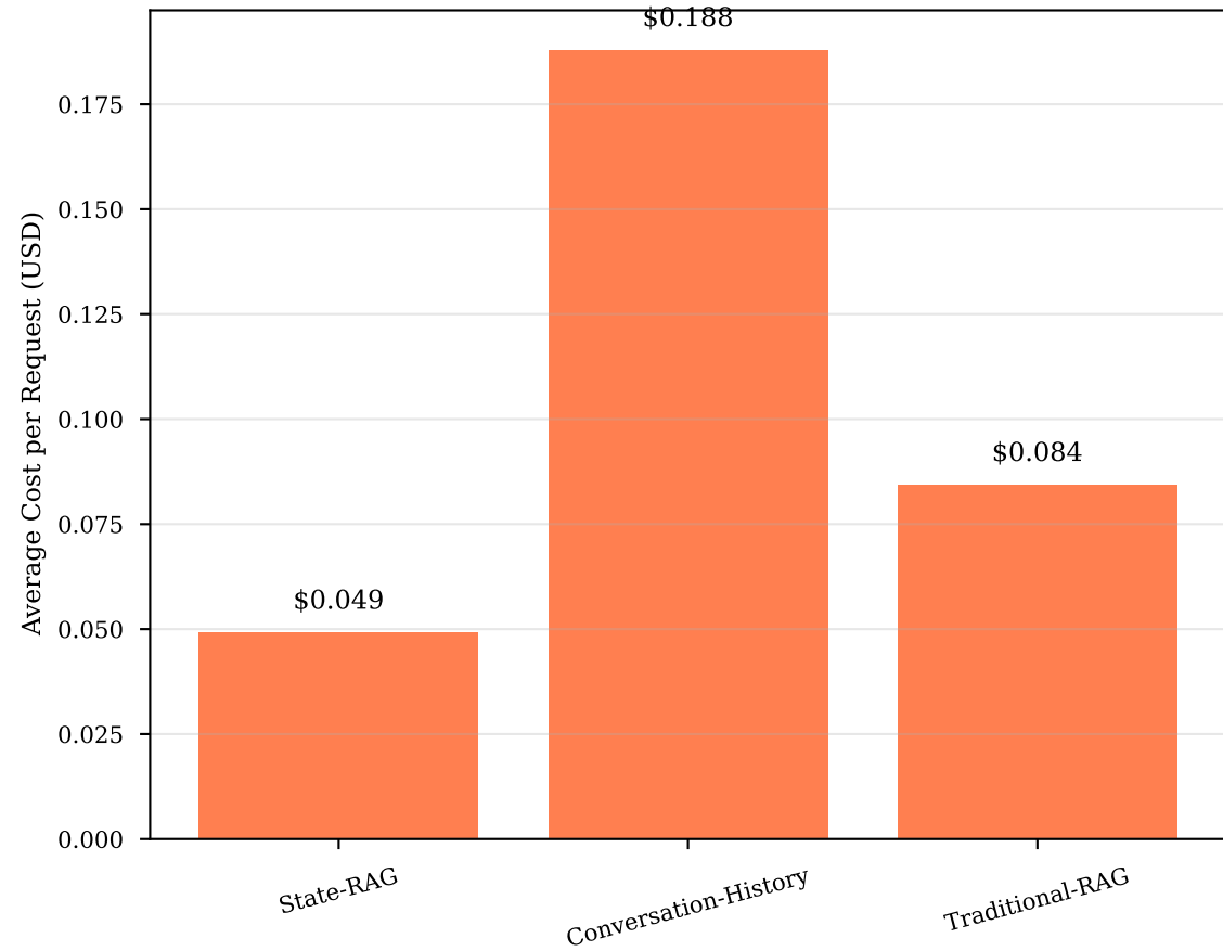
API Cost Comparison
