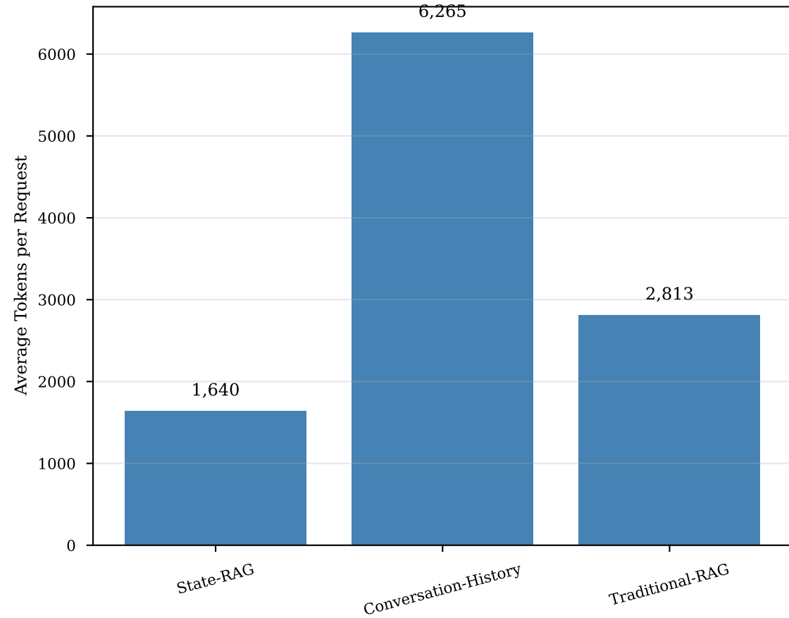
Token Usage Comparison
