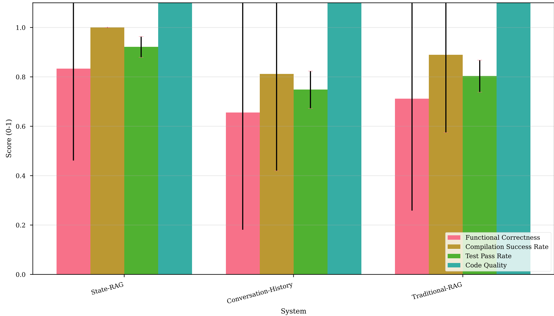
Code Correctness Metrics Comparison
