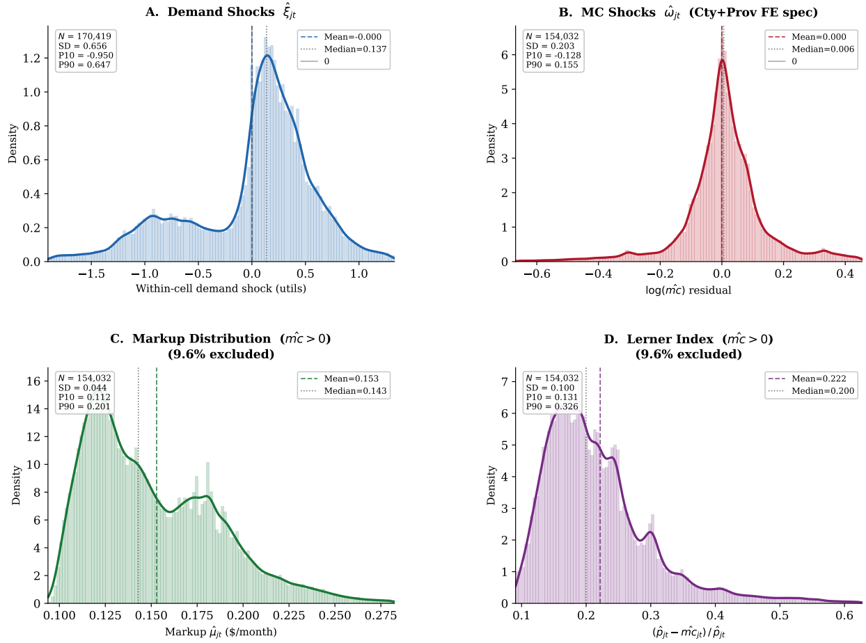
Figure 6: Structural diagnostics from the preferred demand and supply specification (2SLS, County + Provider FEs, Gandhi–Houde instruments). Panel A : kernel density of demand shocks \hat{\xi}_{jt} ; approximately symmetric and centered near zero, consistent with the Gandhi–Houde orthogonality conditions. Panel B : kernel density of marginal-cost shocks \hat{\omega}_{jt} ; symmetric and centered near zero. Panel C : Bertrand–Nash markup distribution; right-skewed with median near $14.3, the elevated right tail driven by multiproduct firms. Panel D : Lerner index distribution; median 0.200, consistent with the inverse-elasticity benchmark 1/|\varepsilon| = 1/4.99 = 0.200 .
