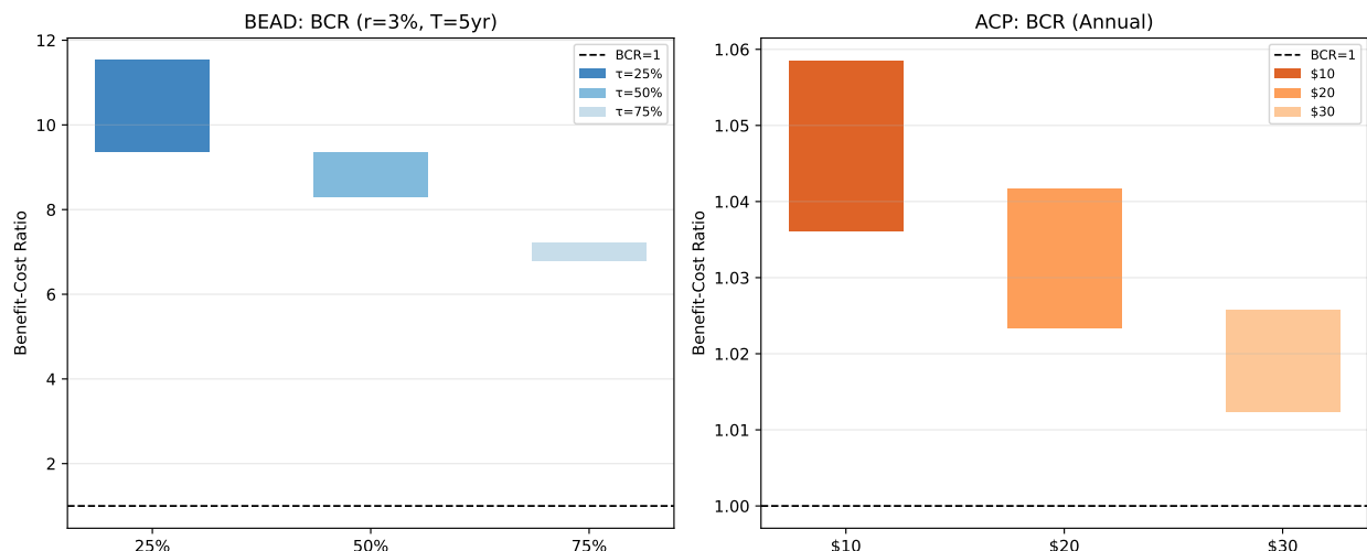
Figure 9: Benefit-cost ratio bounds for BEAD (left, r = 3\% , T = 5\text{ yr} ) and ACP (right, annual flows). Each bar spans [Q_{2.5}, Q_{97.5}] across 50 fixed-cost draws; bar height is parameter uncertainty. Dashed line at \text{BCR} = 1 . BEAD’s one-time government outlay is compared against the discounted five-year welfare stream it funds, so its BCR grows with the horizon and falls with the discount rate (Appendix L). BEAD’s BCR declines with the subsidy rate, from 9.36–11.53 at 25 percent to 6.80–7.22 at 75 percent, reflecting diminishing returns; every bar lies far above 1 and well above ACP’s ratio. ACP BCR is uniformly above 1 across all discount levels and draws, consistent with ACP approximately breaking even on fiscal efficiency while delivering a small positive net surplus. Note the different vertical scales: the ACP bars lie within a range of about 0.05, the BEAD bars within a range of about 4.7.
