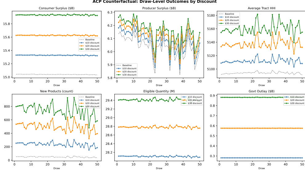
Figure J.3: ACP Counterfactual Outcomes Across Fixed-Cost Draws
