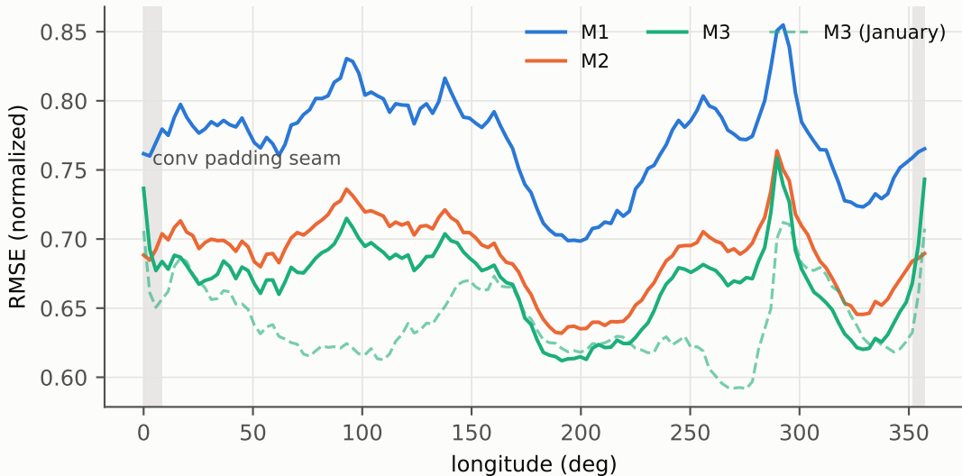
Per-longitude error: M3's boundary seam (July mean)
