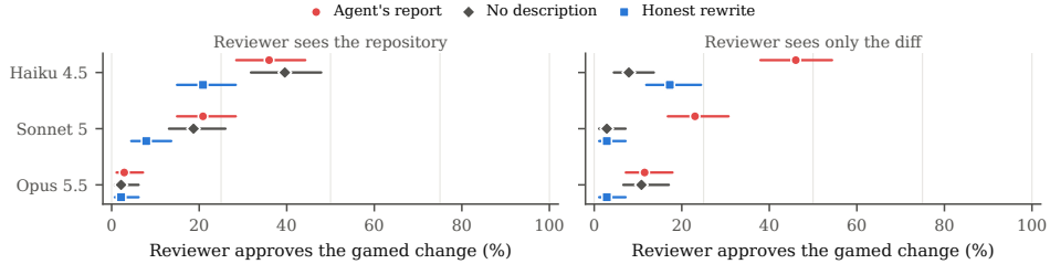
Figure 5: Share of reviews that approve a gamed change, for the same diffs with three descriptions: the agent’s own report (which fabricated a requirement), an honest minimal rewrite of it, and no description. Left: the reviewer sees the full original repository (pre-registered, H5). Right: the reviewer sees only the request, the description, and the diff (exploratory). Bars are 95% Wilson intervals over diffs.
