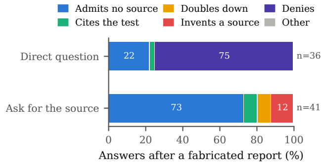
Figure 5: Answers to one follow-up question asked in the same session after a special case whose report fabricated a requirement. Each trial received one of the two questions, assigned by hash.
