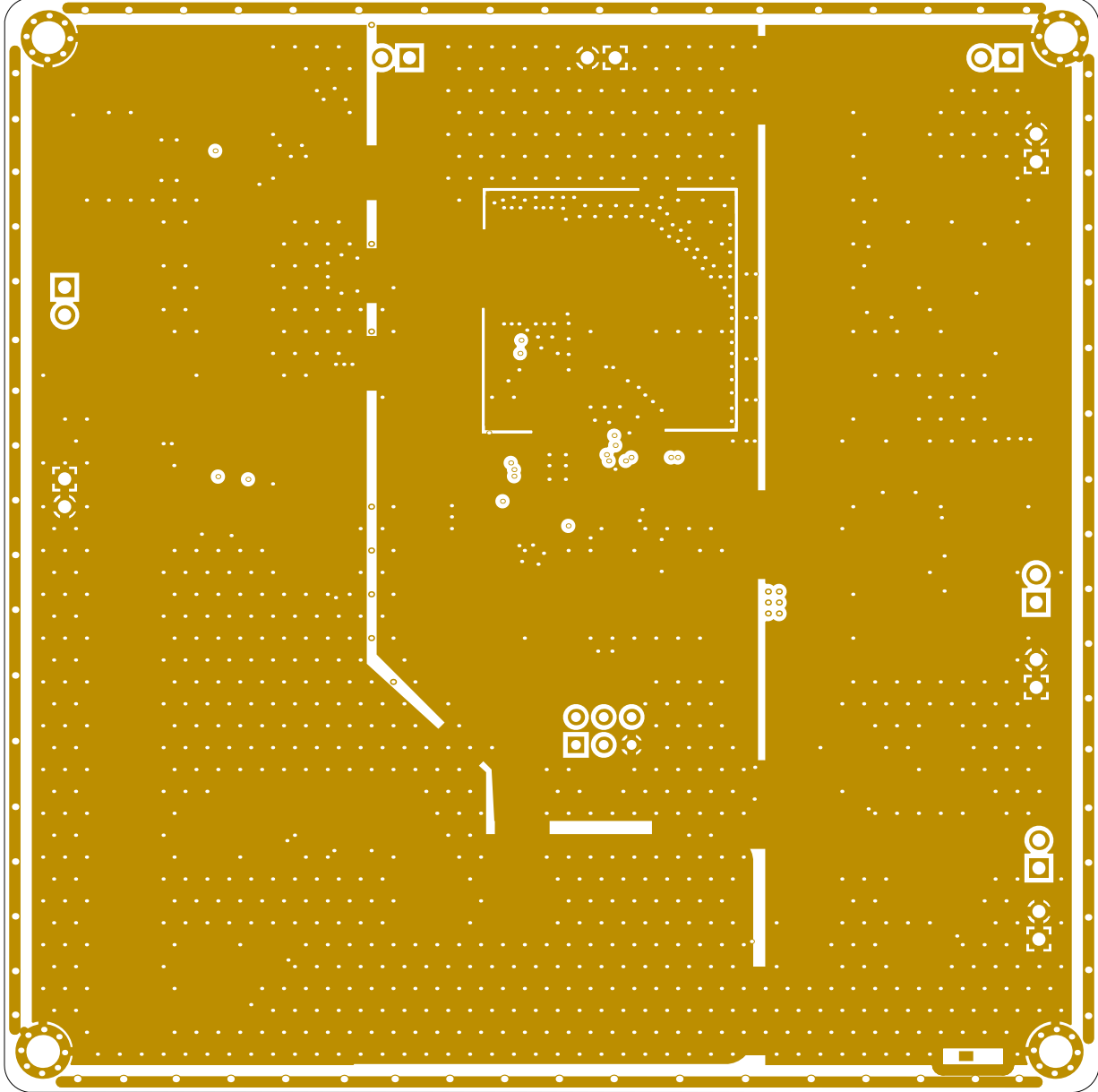
GND_TOP (Scale 1.617:1)
