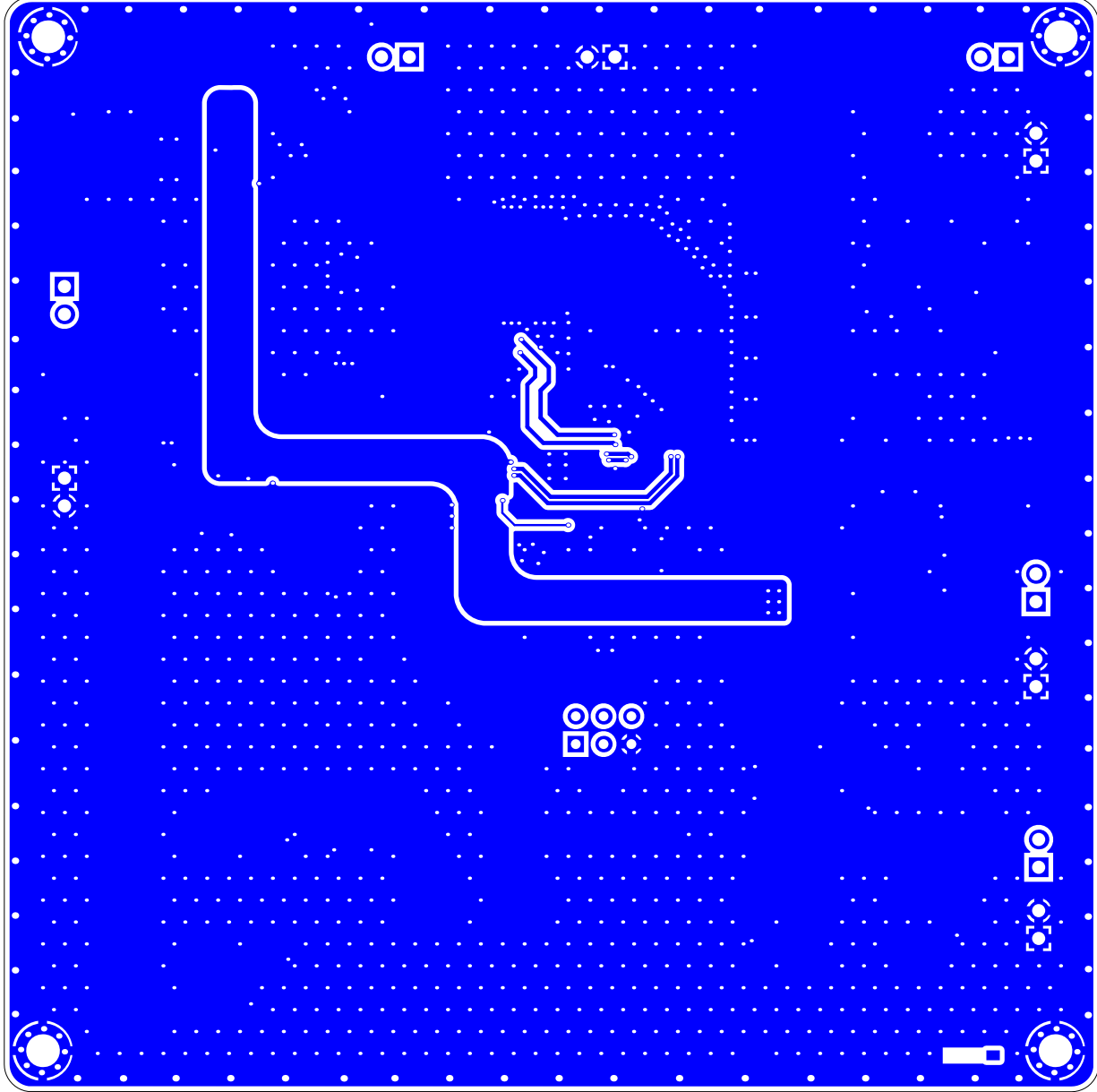
SIGNAL (Scale 1.617:1)
