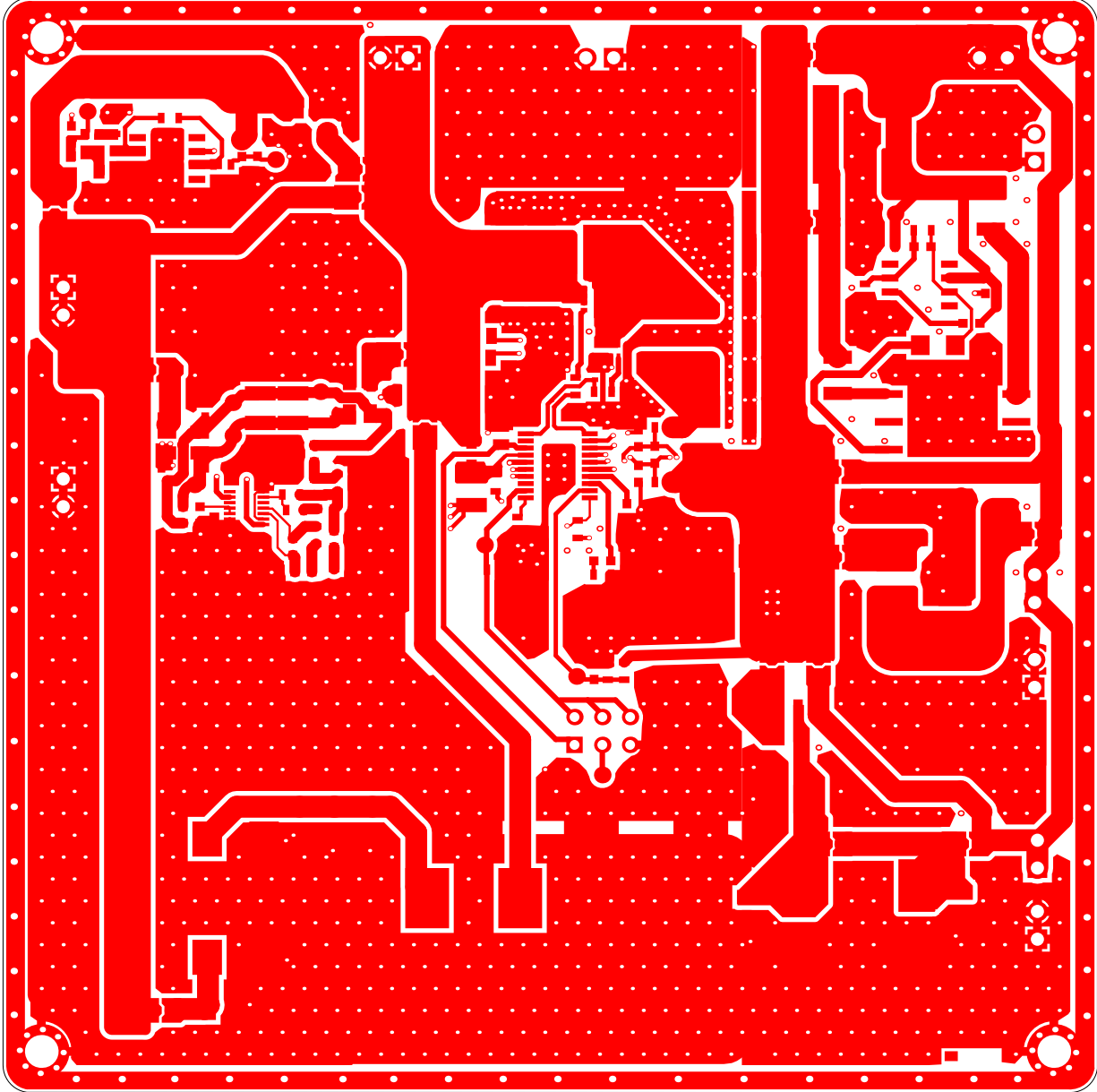
TOP (Scale 1.617:1)
