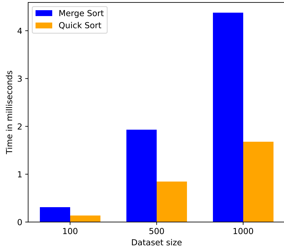
Random
