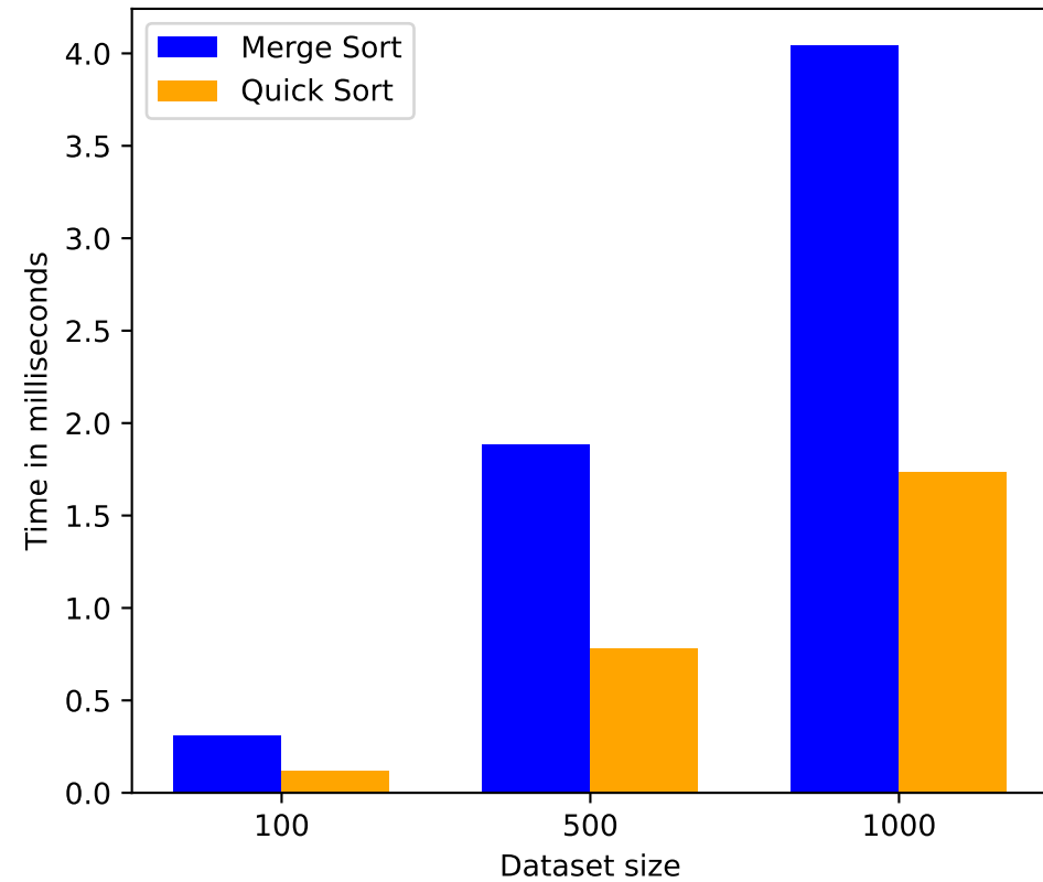
Reversed
