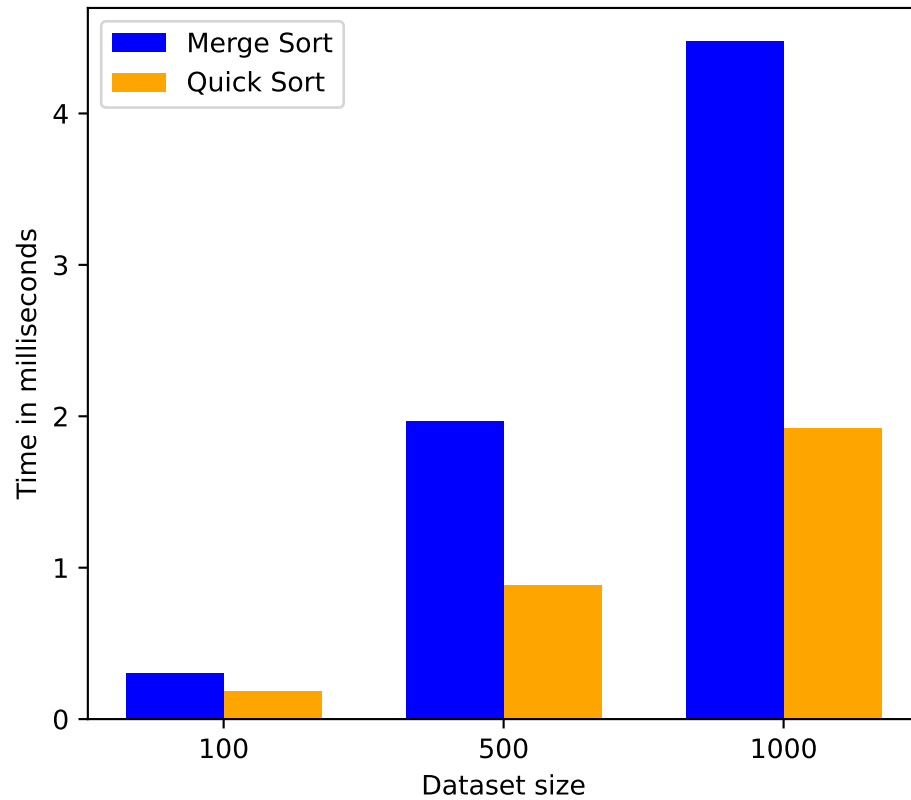
Nearly Sorted
