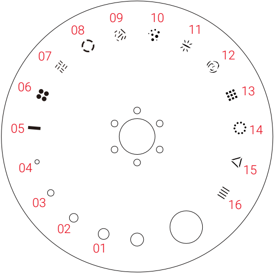
Static Gobo Wheel
