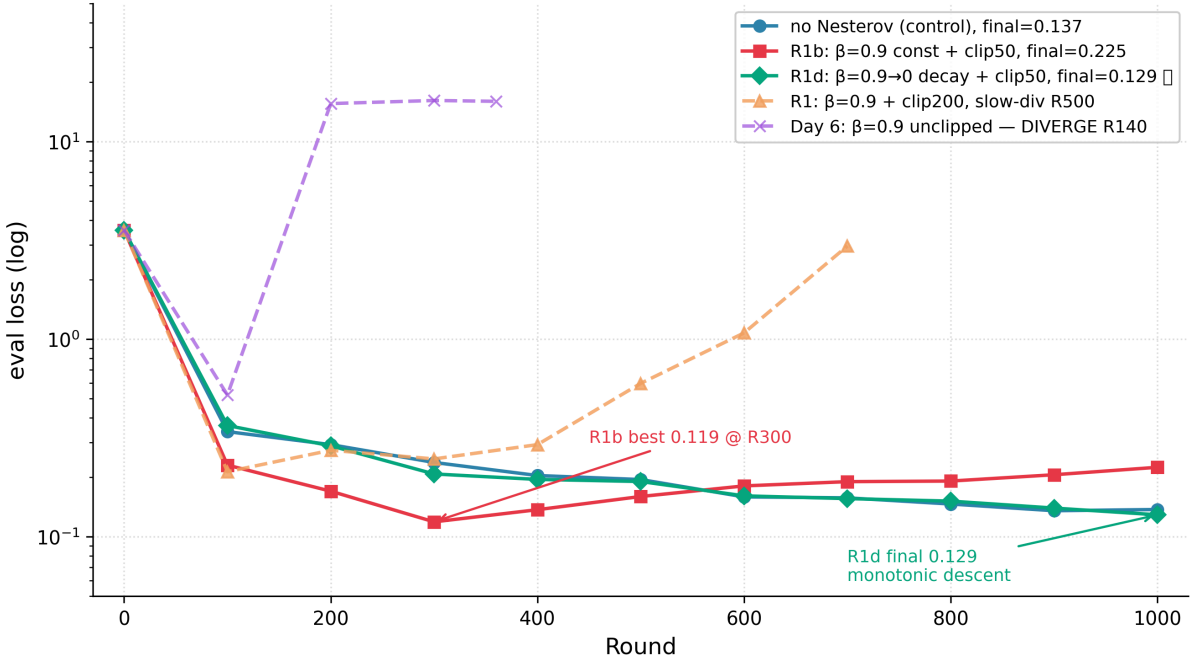
Figure 2. Nesterov-MeZO phase diagram on worst Day 5 cell (ring(4) + Dir( \alpha=0.5 )) All runs at seed=42 for bit-exact ablation; p-clip + \beta -decay required for stable acceleration
