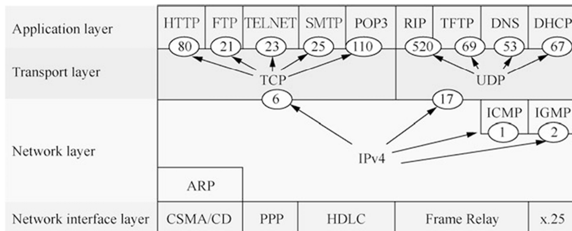
Fig. 2.32 TCP/IPv4 protocol stack
