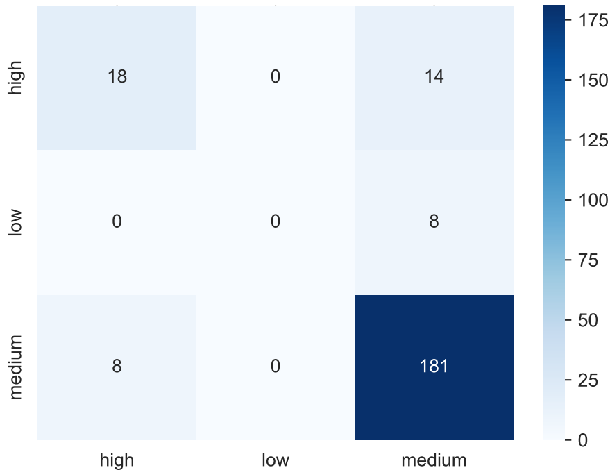
Confusion Matrix — RandomForest
