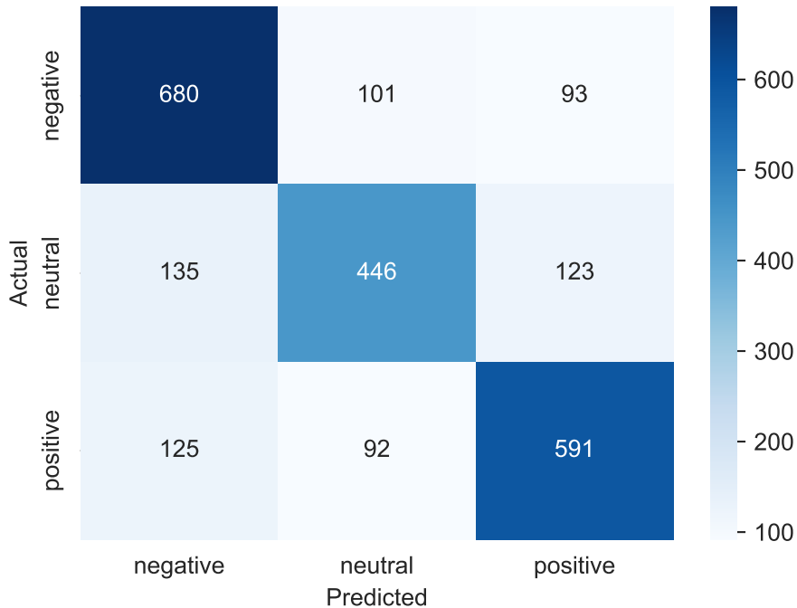
Confusion Matrix — LinearSVC
