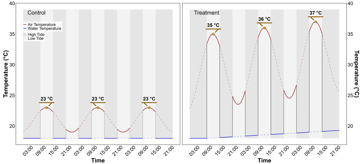
Figure 12: Annexe A2: Temperature profiles of both the control (left) and the treatment (right) followed during the heatwave experiment. The red line indicates air temperature, whereas the blue line indicates water temperature. Due to the tidal cycle followed during the experiment, the seagrasses only experience temperatures represented by solid lines.
