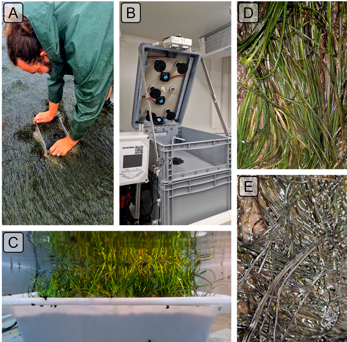
Figure 1: Example of the various steps of the experiment. A: Field sampling of seagrass using a sampling box; B: Intertidal chambers used during the experiment; C: Seagrass sample inside a chamber during the experiment at high tide; D: Photo of the treatment sample at the start of the experiment; E: Photo of the treatment sample at the end of the experiment.
