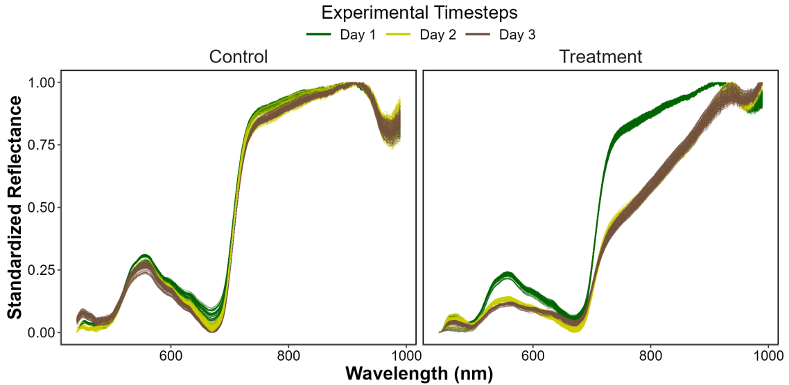
Figure 5: Standardized Hyperspectral Reflectance signature collected during the experiment for both the Control (Left) and the Treatment (Right). Color denotes the progression along the experiment from the beginning (Day 1: green), middle (Day 2: Yellow) and end (Day 3: Brown). A min-max standardization has been applied to each individual spectrum.
