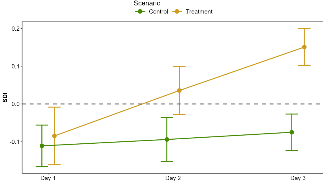
Figure 7: Average and standard deviation of the Seagrass Darkening Index (SDI) across experimental runs, at each day of the experiment. The green line shows values of the Control group while the golden line indicates values of the Treatment group.
