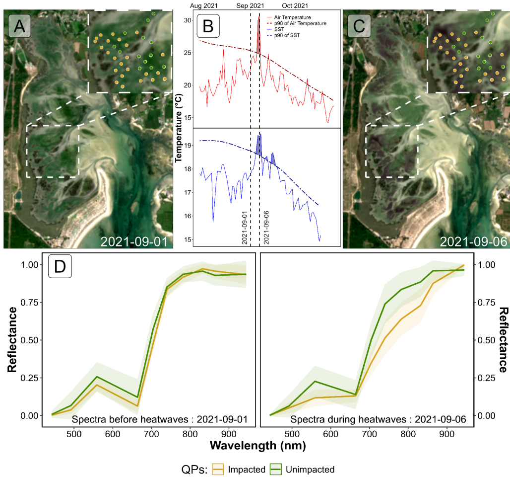
Figure 8: Spectral Comparison of Sentinel-2 Reflectance (D) of Quadrats Points (QPs) Before (A) and During (C) Heatwave Events (B); A: RGB color composition of the Sentinel-2 image on the 1st of September 2021. The points correspond to QPs collected on September 10, 2021, with unimpacted seagrass in green and impacted seagrass in golden; B: Detection of heatwave events based on both Air Temperature and Sea Surface Temperature (SST). The solid line represents the daily average temperature, while the dashed line indicates the 90th percentile of the climatology. Colored areas identify heatwaves (marine in blue and atmospheric in red). The two vertical dashed lines represent the acquisition dates of the two Sentinel-2 images used in this analysis (01-09-2021 and 06-09-2021) ; C : RGB color composition of the Sentinel-2 image on the 6th of September 2021, with unimpacted seagrass in green and impacted seagrass in golden; D : Average spectral signatures of QPs where dark and green seagrasses (gold and green lines, respectively) were identified during the field survey. The left plot shows the reflectance of these QPs before the heatwave impact, while the right plot shows the spectral signature during the heatwaves. The ribbons around the lines represent the standard deviation.
