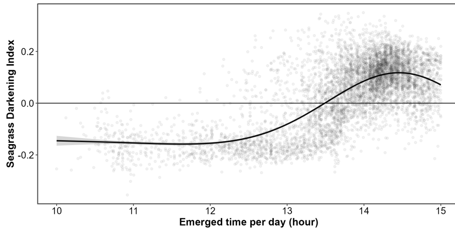
Figure 12: Seagrass Darkening Index as a function of the daily emergence time of seagrasses. The line represents a Generalized Linear Model (GLM) prediction, and the shaded area indicates the standard error. Shaded points represent raw data, with each point corresponding to a single pixel.
