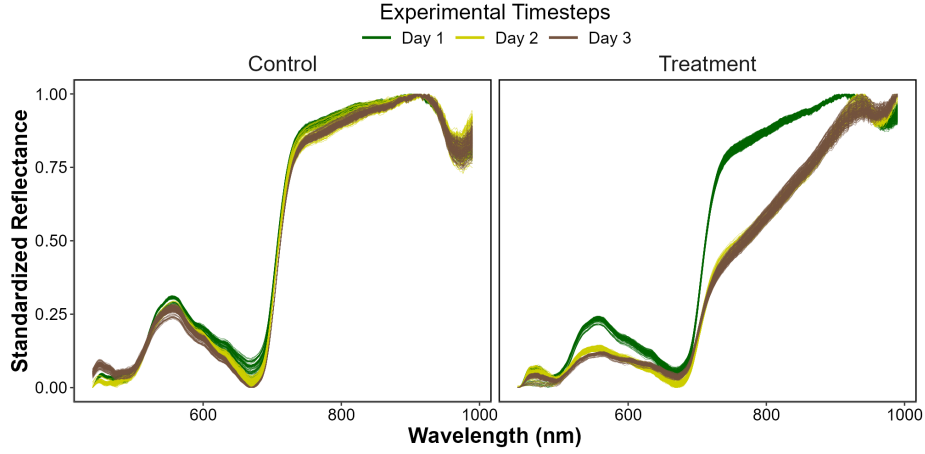
Figure 6: Standardized Hyperspectral Reflectance signature collected during the experiment for both the Control (Left) and the Treatment (Right). Color denotes the progression along the experiment from the beginning (Day 1: green), middle (Day 2: Yellow) and end (Day 3: Brown).
