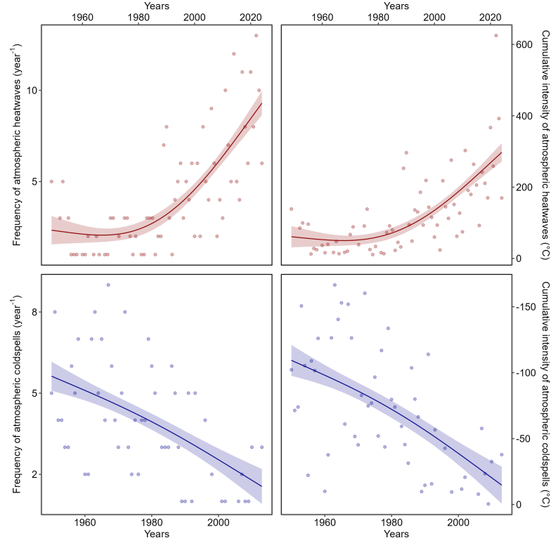
Figure 10: Frequency and intensity of atmospheric heatwaves (red) and cold spells (blue) over time at the Lorient-Lann Bihoué weather station. The left column displays the annual frequency of heatwaves and cold spells as the total number of events per year. The right column illustrates event intensity, represented by the cumulative temperature anomaly throughout the year, measured in degrees Celsius.
