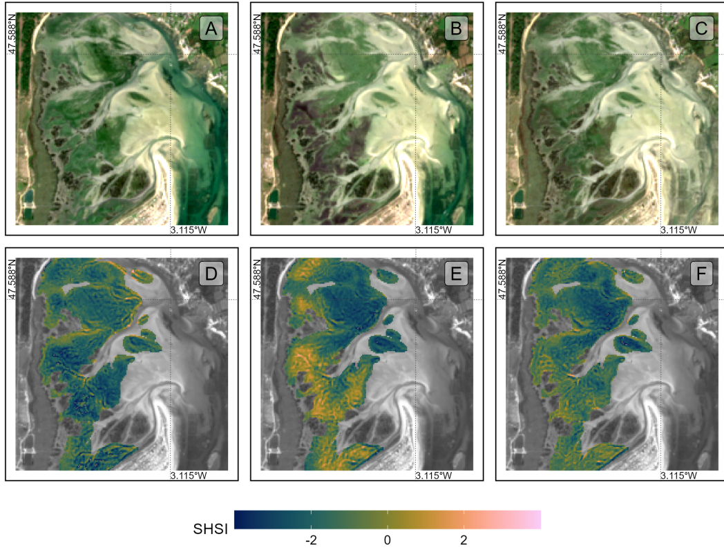
Figure 11: Sentinel-2 color composition of the seagrass meadow of Quiberon, South Brittany, France, Before (A ; 1st of September 2021), During (B ; 6th of September 2021) and After (C ; 8th of October 2021) the HW and SHSI applied to the same Sentinel-2 images Before (D), During (E) and After (F) the HW.
